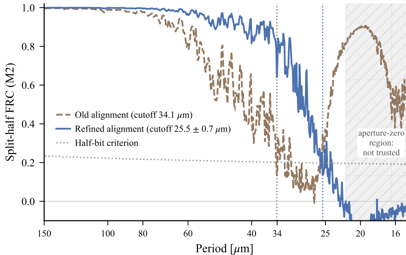
(b) Recoverable band: 34.1 \rightarrow 25.5 \mu\text{m}
