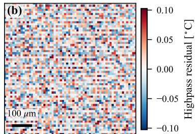
Synthetic x_0 = phase-bin drizzle (ch5, current)
