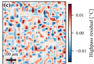
Synthetic x_0 = aligned mean (ch0, de-waffled)
