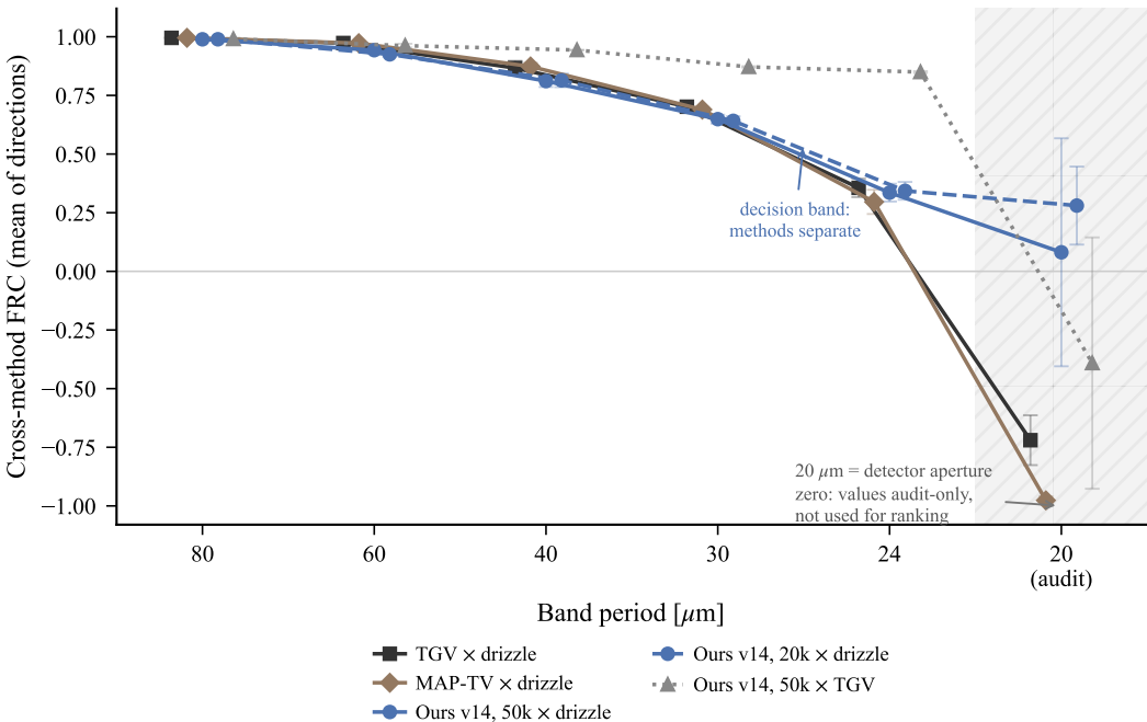
Cross-FRC band table across methods (stage0j leaderboard)
