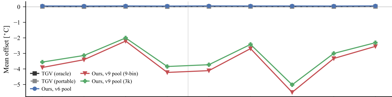
(b) Low-frequency stability
