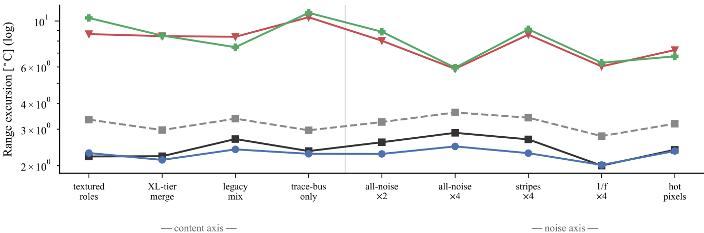
(b) Low-frequency stability
