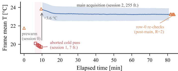
(b) Acquisition timeline & thermal state
