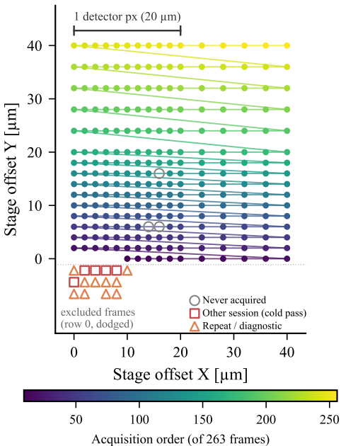
(a) Step-stop raster trajectory
