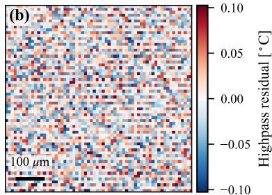
Synthetic x_0 = phase-bin drizzle (ch5, current)
