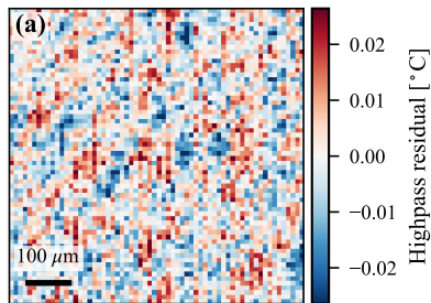
Real drizzle composite (warm start carries this)
