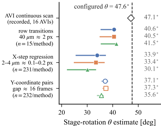
(a) \theta by estimation method
