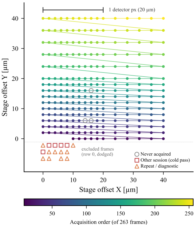
(a) Step-stop raster trajectory
