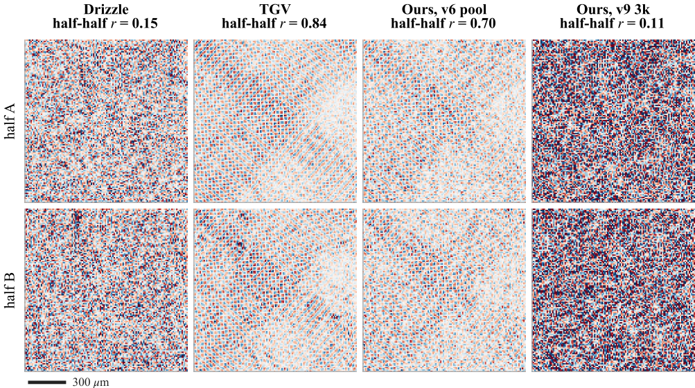
Flat ROI, 25-40 \mu\text{m} band. Split-stable texture (TGV, v6) is what self split-half FRC rewards --- hence cross-FRC vs drizzle as metrology (fig31/32).
