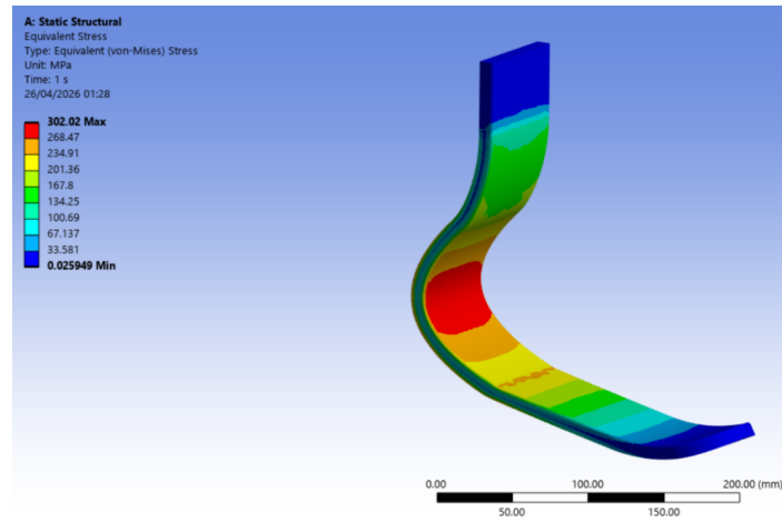
Figure 8: Von Mises stress distribution for Design 2 CFRP. Peak stress 302.02 MPa, a 25.1% reduction from Design 1.
