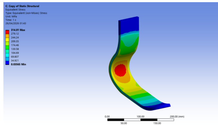
Figure 11: Von Mises stress distribution for Design 2 Aluminium 2014 T4. Peak stress 314.01 MPa exceeds yield strength of 270 MPa.
