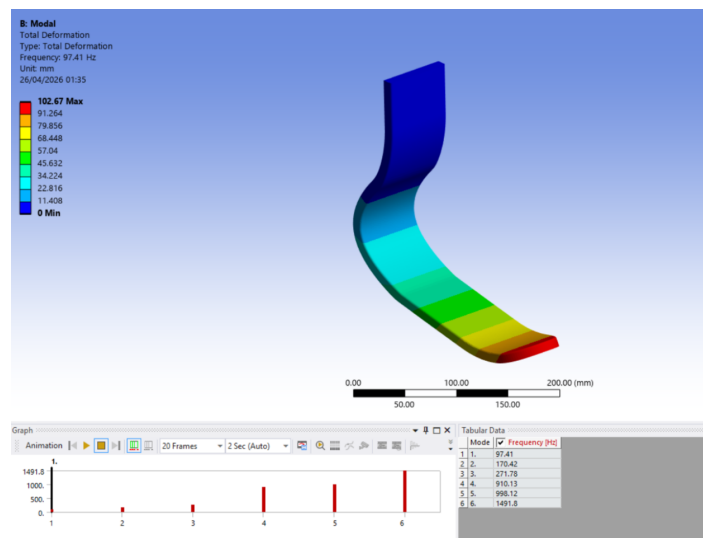
Figure 9: Mode shape 1, natural frequency
