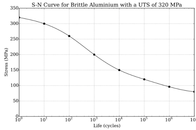
Figure 3: Aluminium 2014 T4 S-N Curve
