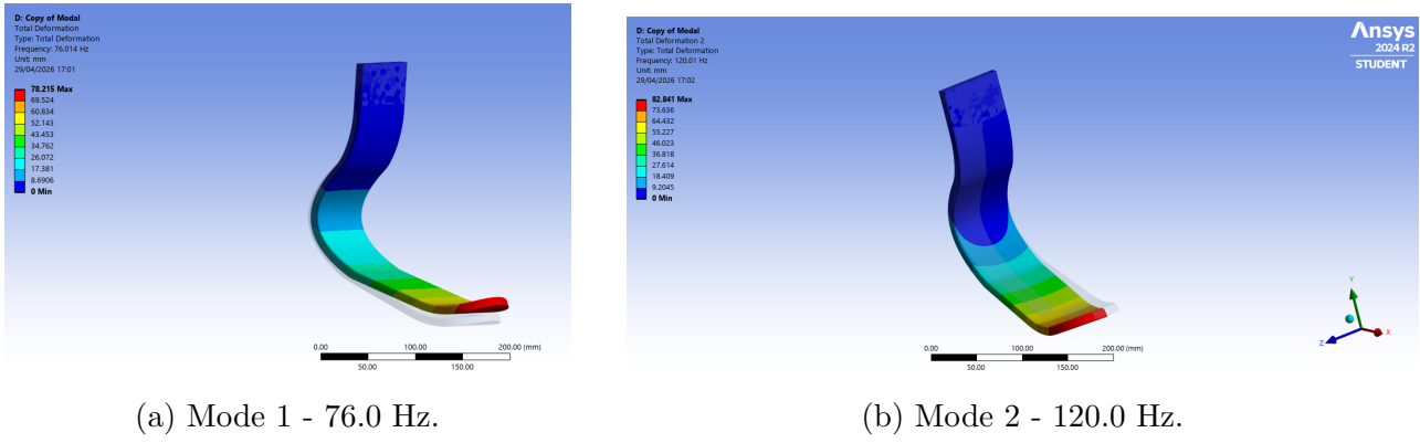
Figure 12: Mode shapes for Design 2 Aluminium 2014 T4.
