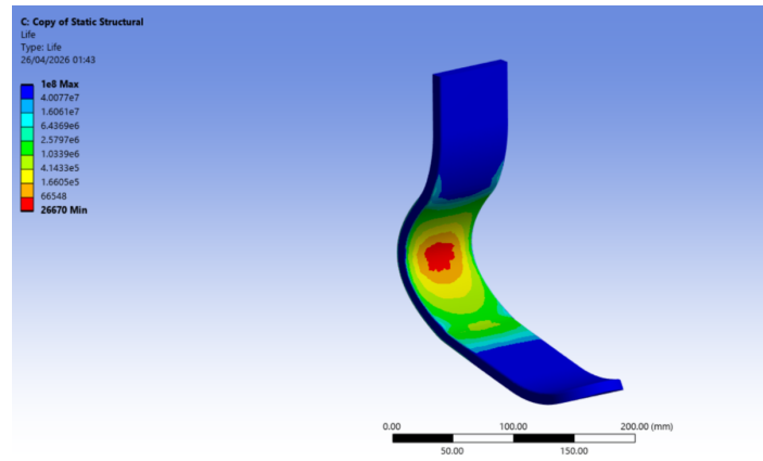
Figure 10: Fatigue life contour for Design 2 Aluminium 2014 T4. Minimum life 26,670 cycles at inner curve radius. Red zone indicates region of earliest fatigue failure.
