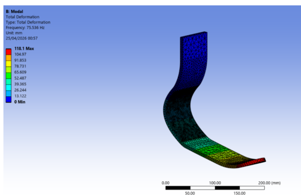
(a) Mode 1 - 75.5 Hz.
