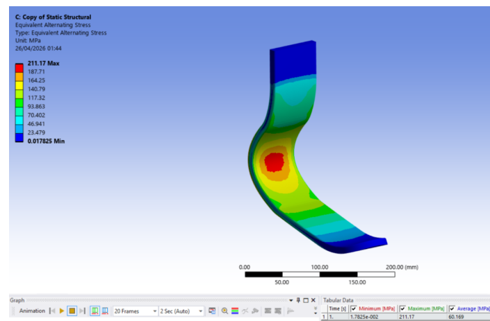
Figure 13: Aluminium, alternating stress
