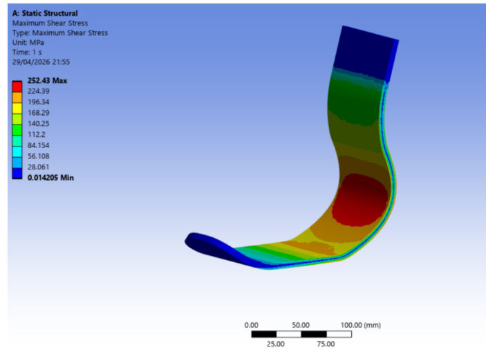
Figure 14: Design 1 CFRP Shear Stress
