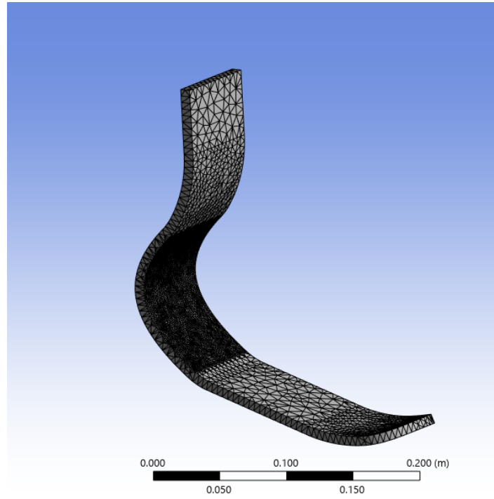
Figure 5: Final converged mesh for Design 1
