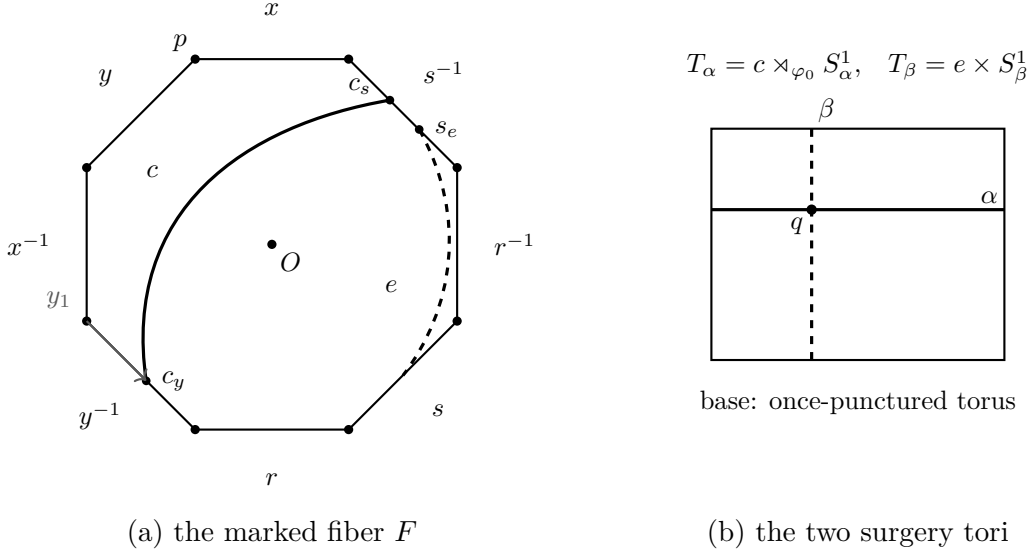
Figure 1: The marked data reconstructed by the audit. Panel (a) is the symmetric octagon model of the genus-two fiber, with boundary word xyx^{-1}y^{-1}rsr^{-1}s^{-1} ; all eight corners represent the basepoint p , while O is the center. Half-turn carries opposite edges to one another and induces x \leftrightarrow r , y \leftrightarrow s . The displayed arcs record the curve c , the five-chain curve e , and the initial y_1 whisker; the corresponding s_2 whisker is stored in the simplicial model. Panel (b) is a schematic of the two curve subbundles over the base loops. The geometric placements are checked as simplicial path and incidence assertions; the drawing is explanatory rather than an additional input to the computation.
