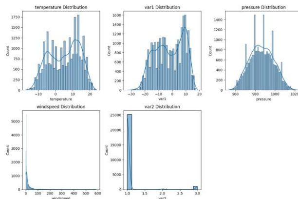
Figure 5: Histograms and Density Plots for Numerical Features
