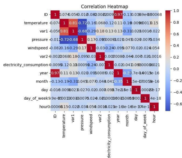
Figure 7: Correlation matrix heatmap
