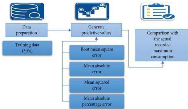
Figure 1: Project flow
