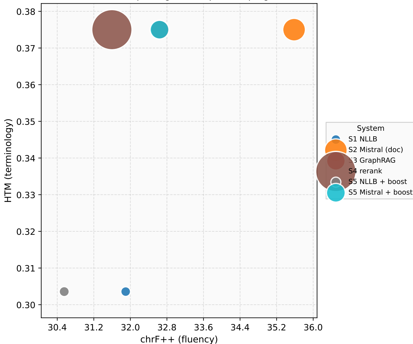
Fluency vs terminology vs computational cost (bubble area \propto mean seconds per segment — prefer top-right, smaller bubbles)
