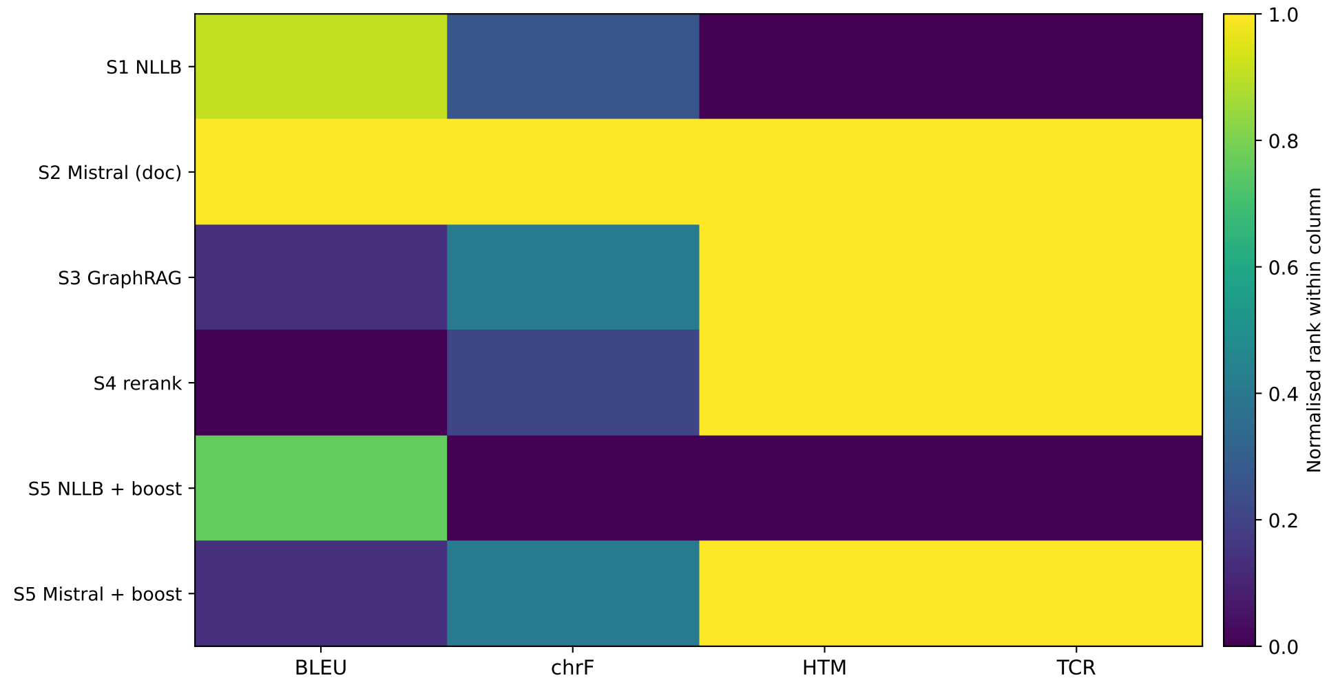
Relative standing per metric (column min-max normalisation)
