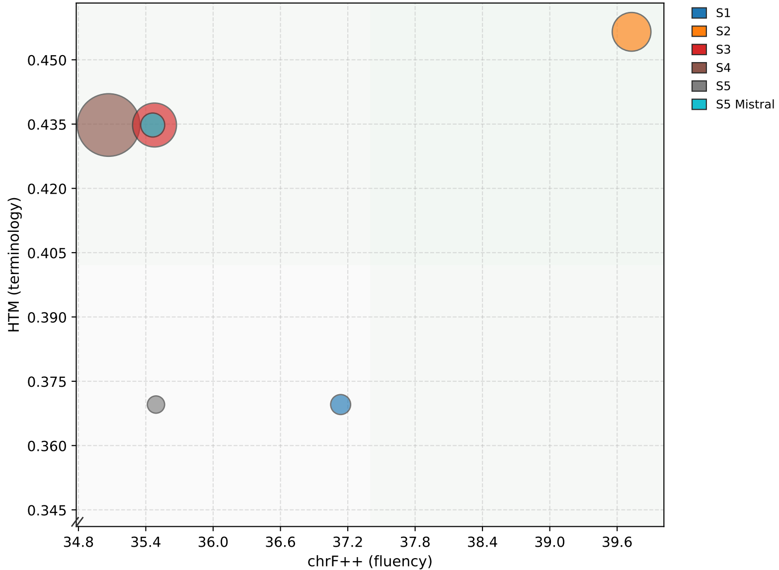
Fluency vs terminology (bubble size \propto mean seconds per segment)
