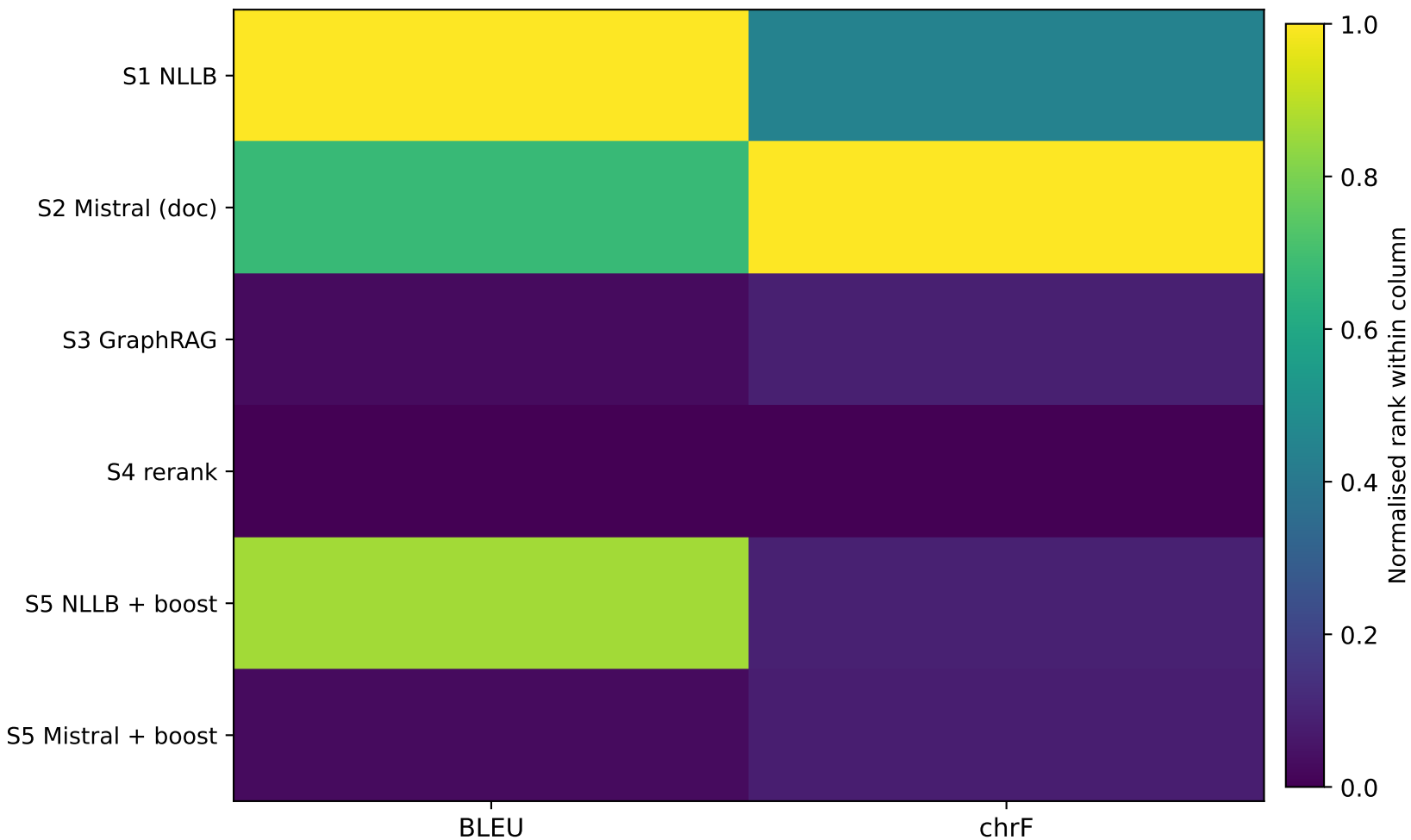
Relative standing per metric (column min-max normalisation)
