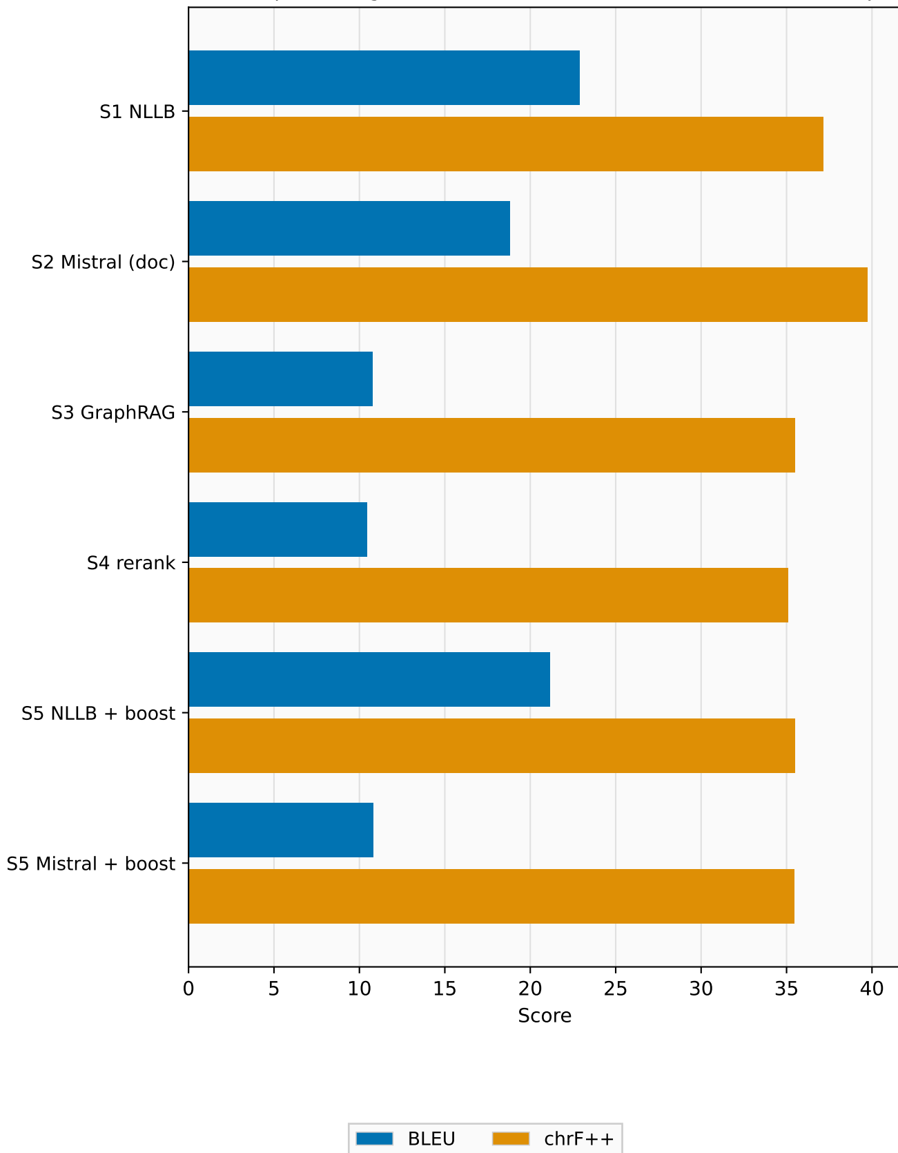
Overlap with English reference (BLEU · chrF++; HTM needs Neo4j)
