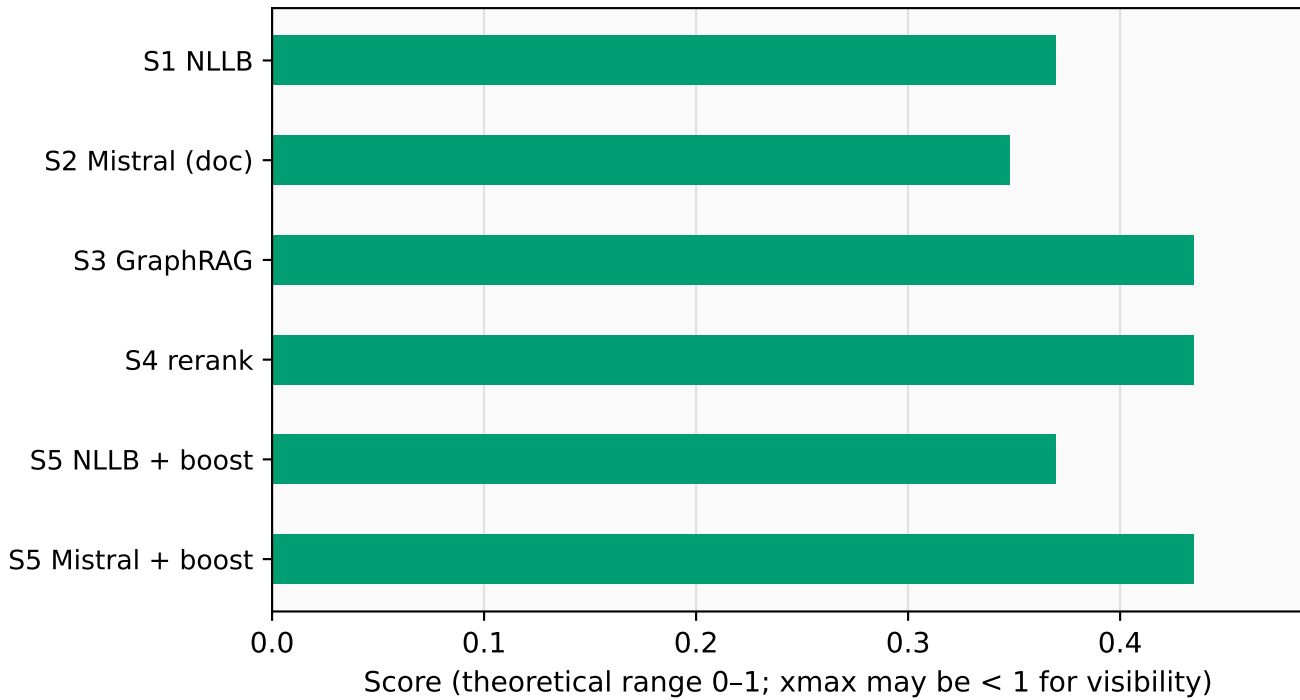
HTM — hierarchy-aware term match (gold_terms + graph; panel zooms when values are small)
