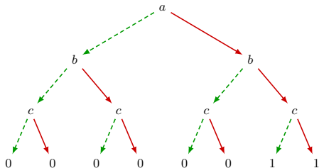
(b) a decision tree (a not reduced BDD)
