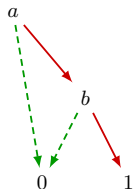
(c) a (reduced) BDD
