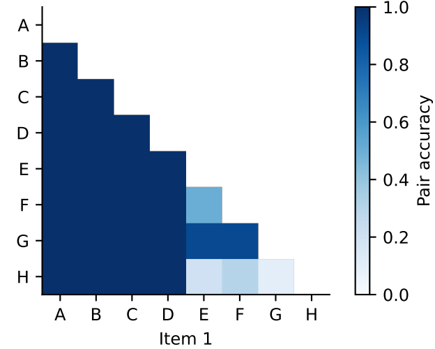
Network 2105 subject 8 G>E>F>H>D>C>B>A
