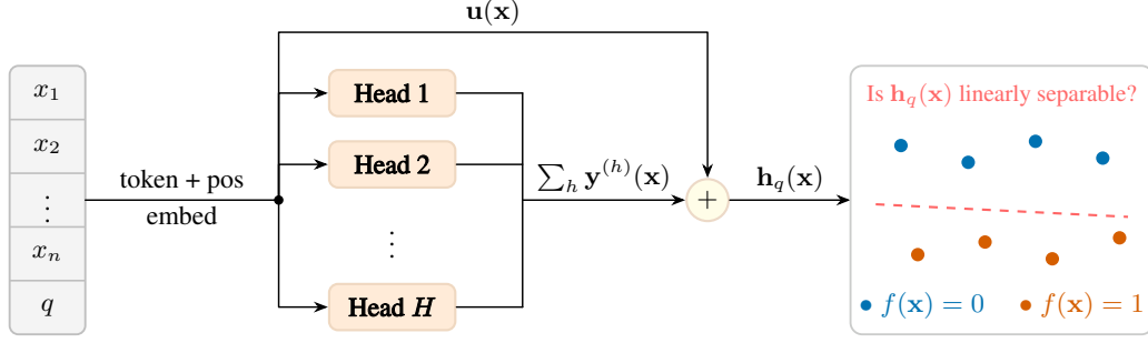
Figure 1: One-layer attention-only model. The input consists of n bit tokens followed by a dedicated query token q , which also serves as the readout position. Each position is represented by the sum of a token embedding and a positional embedding, and the resulting embedded sequence is shared by all H heads. The heads update all positions in parallel, but the linear readout uses only position q . At this position, the head outputs are added to the residual u_q , yielding h_q(\mathbf{x}) . Thus, f is represented exactly when the inputs labelled 0 and 1 are linearly separable at the readout position h_q(\mathbf{x}) , and H^*(f) is the minimum H for which this occurs.
