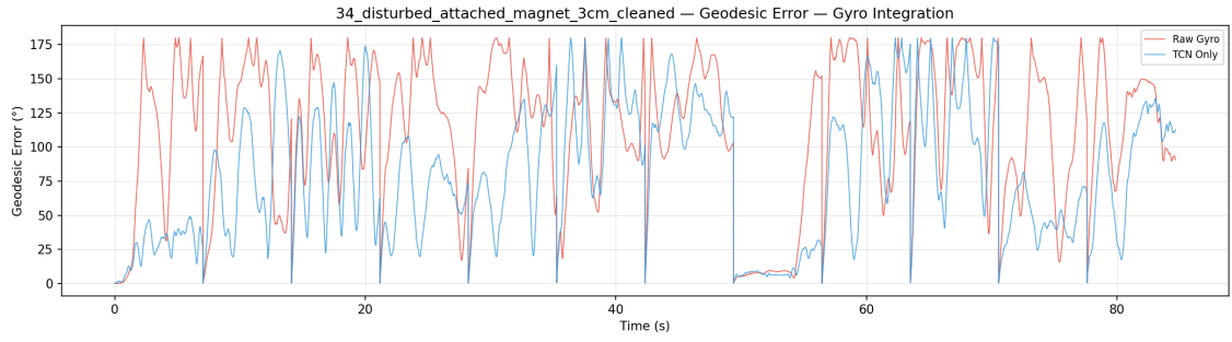
Figure 15: Geodesic Angle Error (dead reckoning) for Trial 34: Disturbed Magnet attached 3cm
