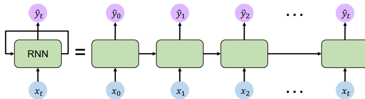
Figure 4: RNN structure [30]
