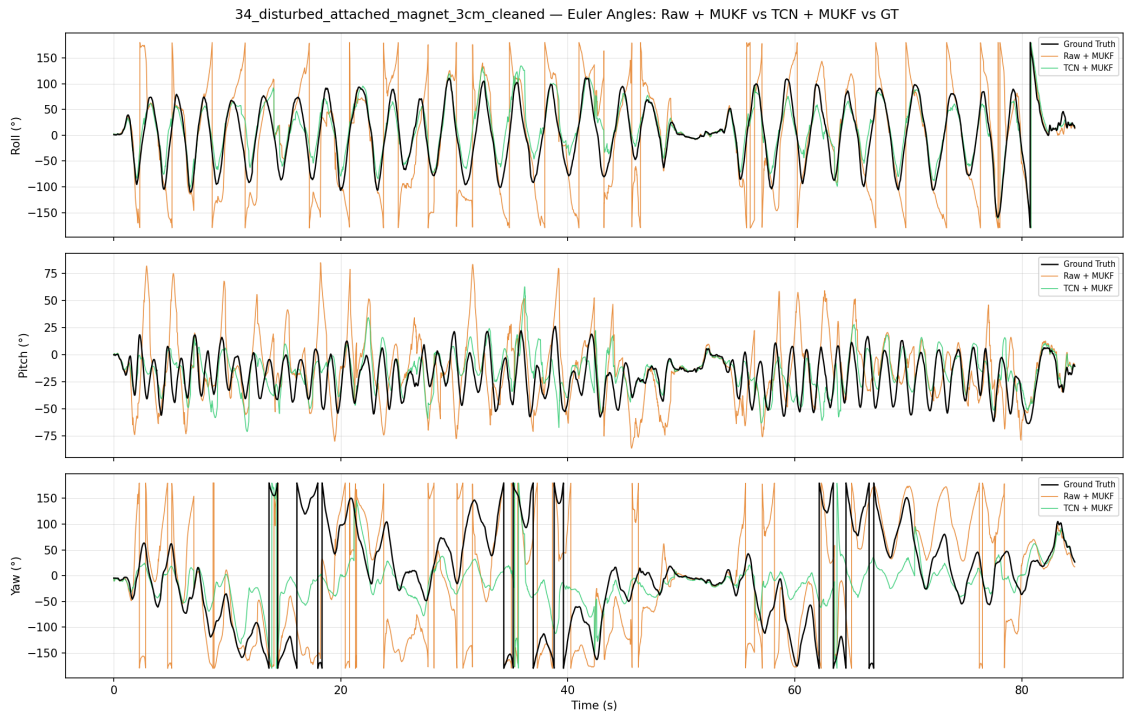
Figure 17: Euler Angle Plots (MUKF pipeline) for Trial 34: Disturbed Magnet attached 3cm
