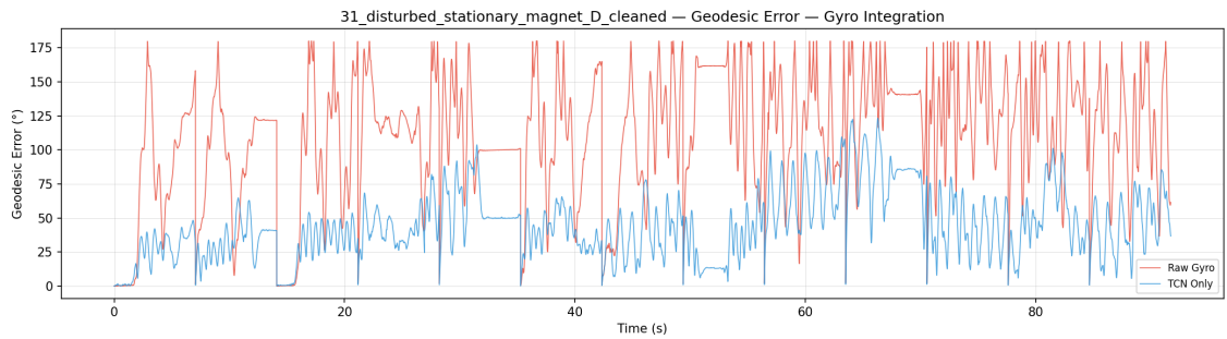
Figure 11: Geodesic Angle Error (dead reckoning) for Trial 31: Disturbed Stationary Magnet
