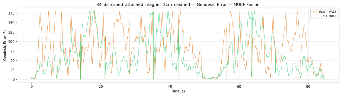
Figure 16: Geodesic Angle Error (MUKF pipeline) for Trial 34: Disturbed Magnet attached 3cm
