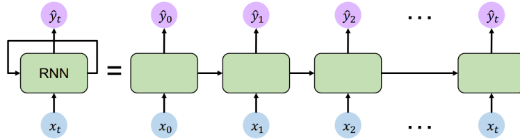
Figure 7: RNN structure [20]
