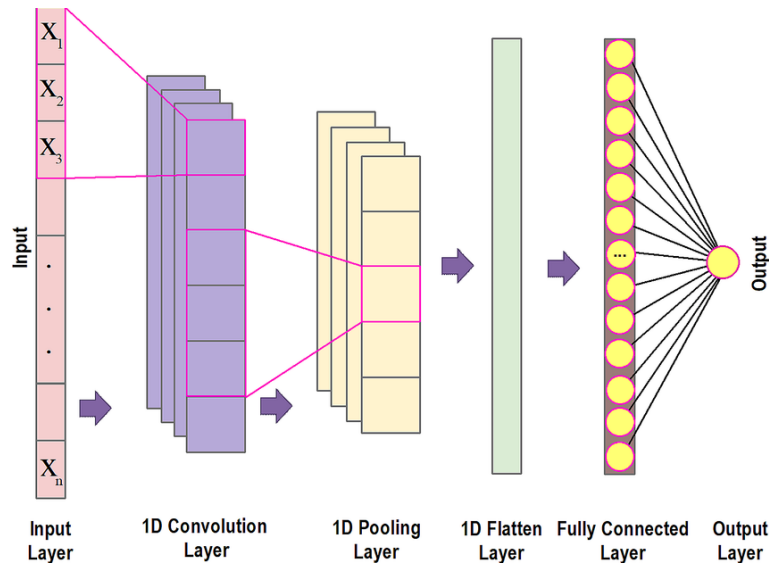
Figure 8: 1D CNN structure [26]
