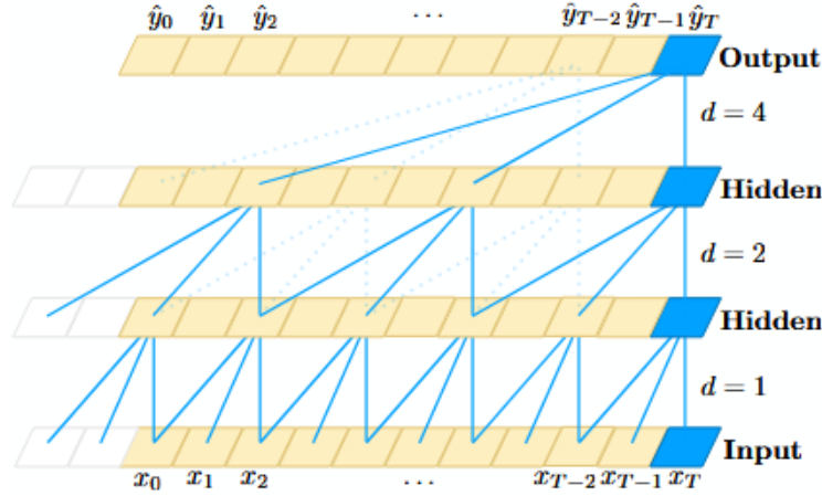
Figure 9: CNN structure with dilations [28]
