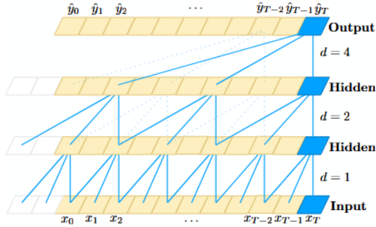
Figure 5: CNN structure with dilations [30]
