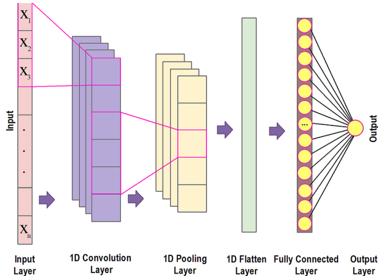
Figure 4: 1D CNN structure [28]
