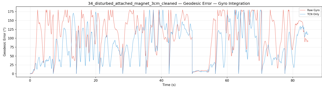
Figure 17: Geodesic Angle Error (dead reckoning) for Trial 34: Disturbed Magnet attached 3cm
