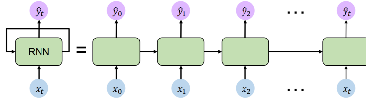
Figure 4: RNN structure [30]
