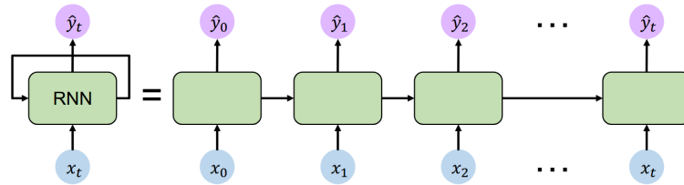
Figure 4: RNN structure [30]
