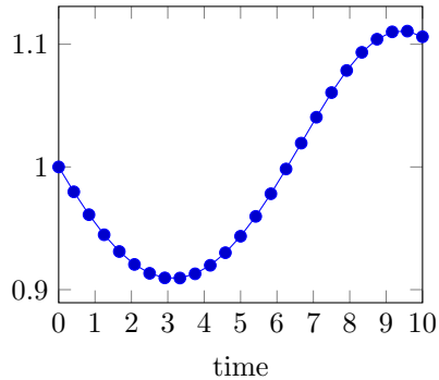
Marginal utility u'(c_t)
