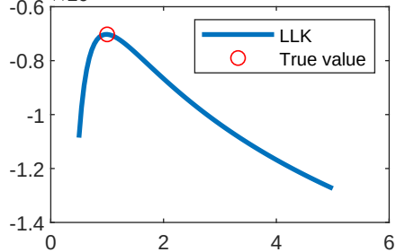
LLK function for different \sigma
