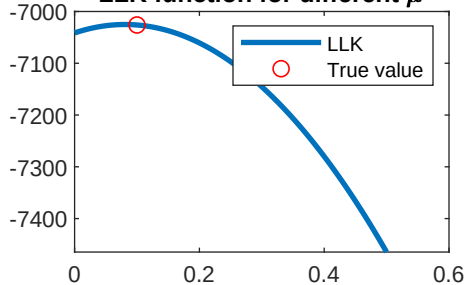
LLK function for different \mu
