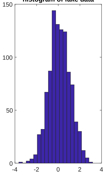
histogram of fake data
