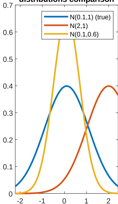
distributions comparison
