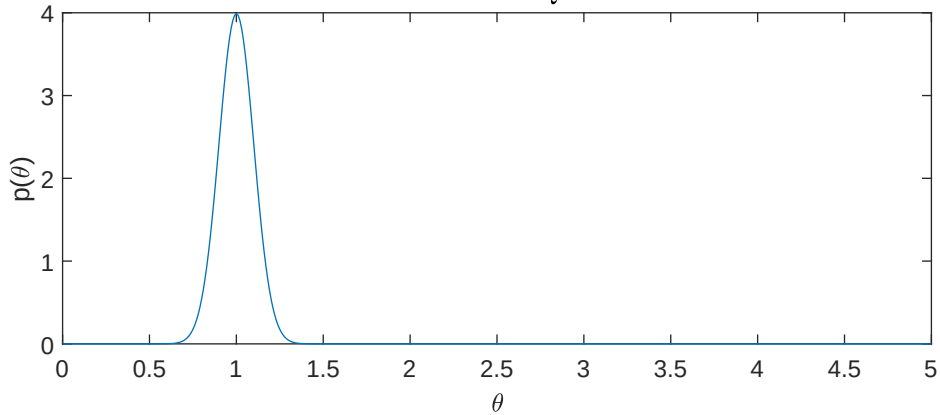
Prior for \hat{Q}
