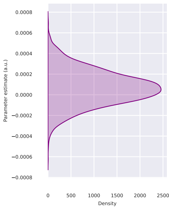
Non-dec time - InattentionW (high OV) p=0.344
