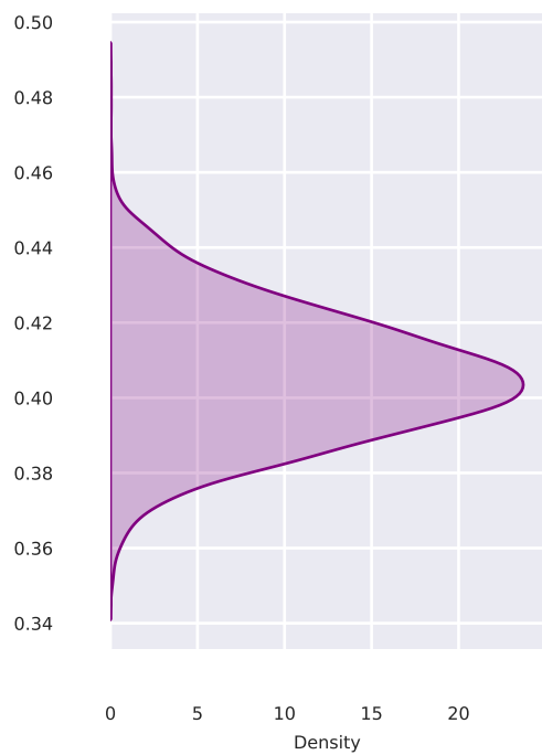
Non-dec time (intercept) p=0.000
