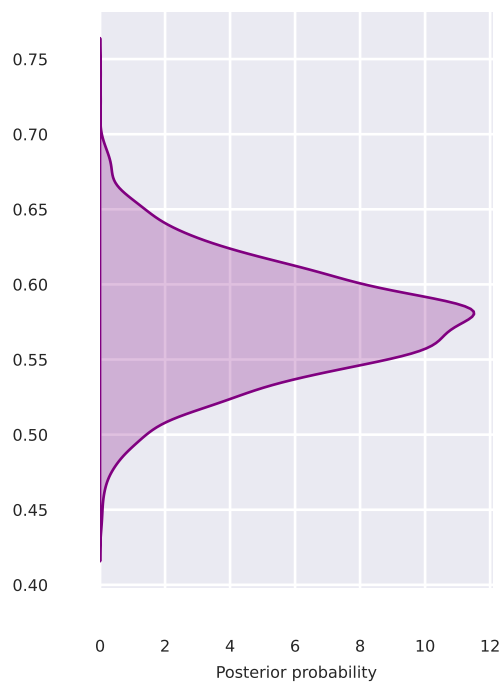
Intercept drift rate p=0.000
