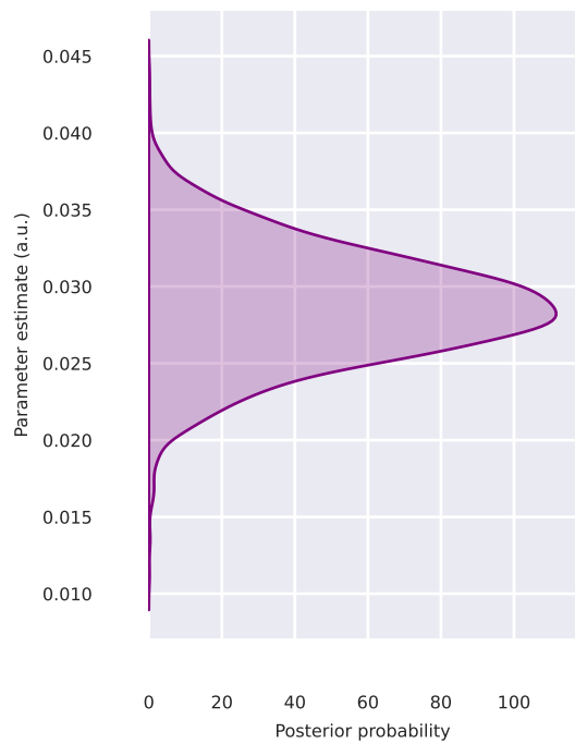
Drift - InattentionW (high OV) p=0.000
