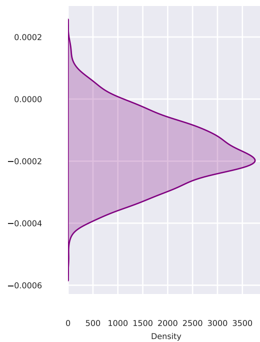
Non-dec time - InattentionW (med OV) p=0.062
