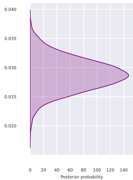
Drift - AttentionW p=0.000
