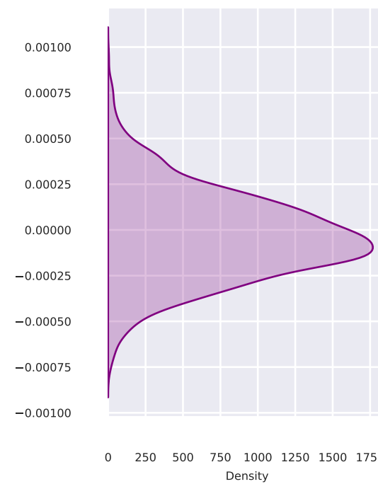
Non-dec time - InattentionW (low OV) p=0.414
