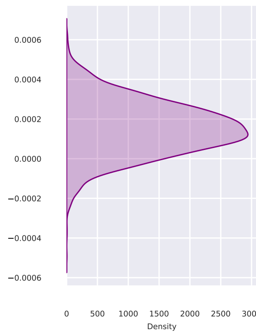
Non-dec time - AttentionW p=0.120
