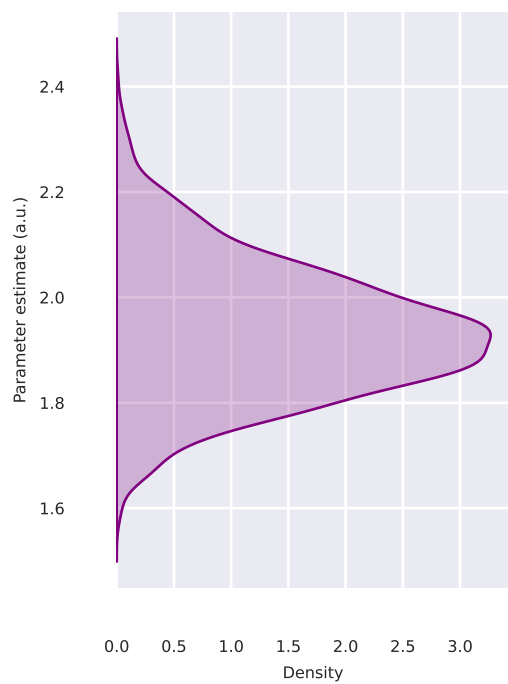
Boundary sep. p=0.000
