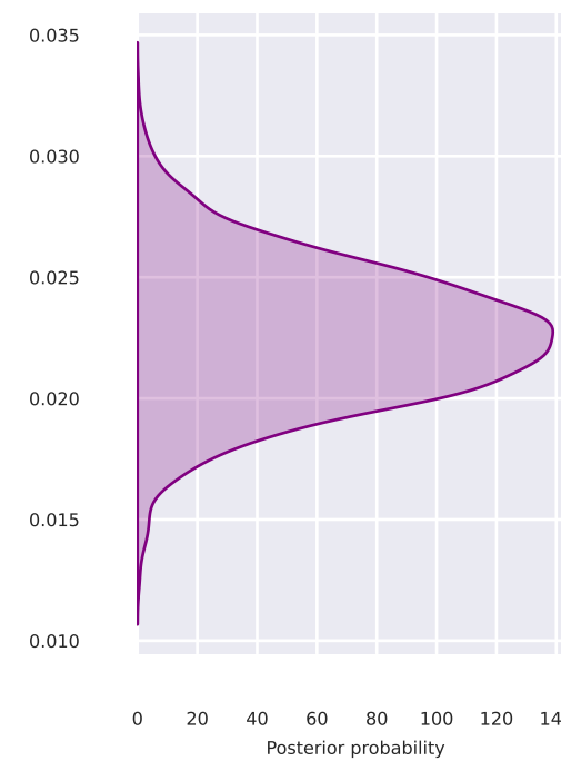
Drift - InattentionW (low OV) p=0.000
