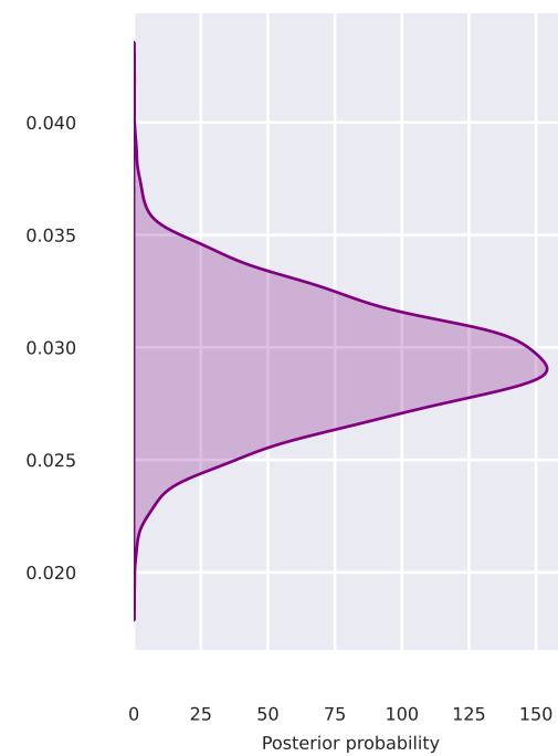
Drift - InattentionW (med OV) p=0.000
