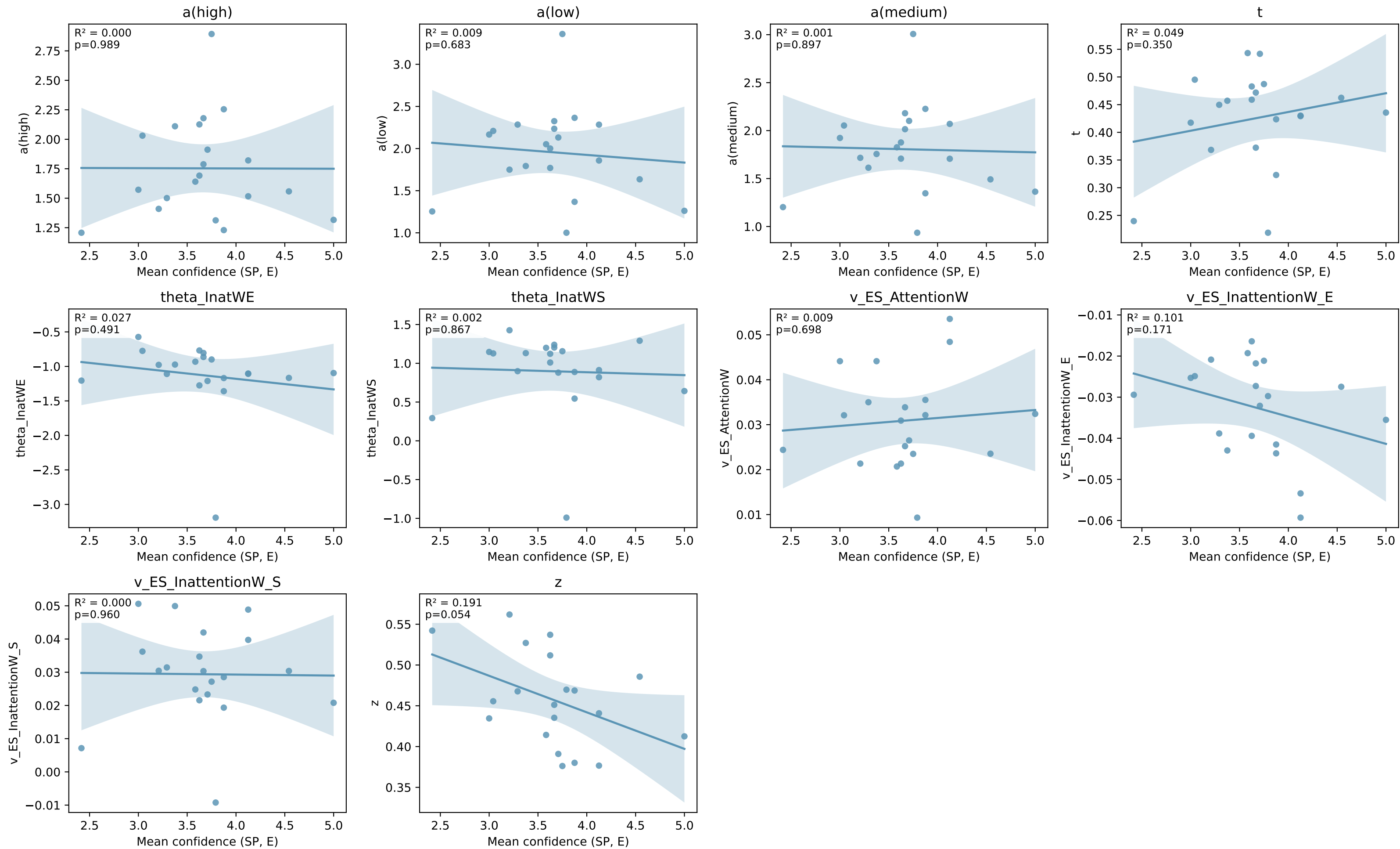
Correlations: SP confidence (E) vs aDDM parameters
