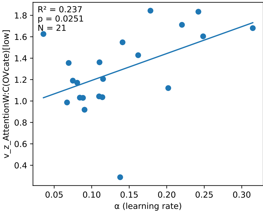
v_z_AttentionW:C(OVcate)[low]
