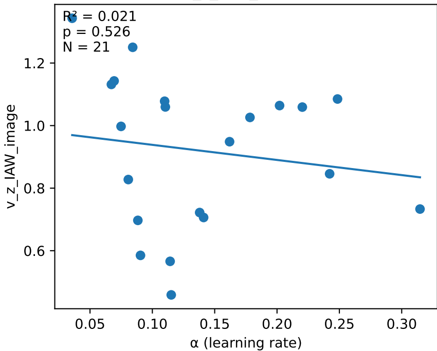
v_z_IAW_image
