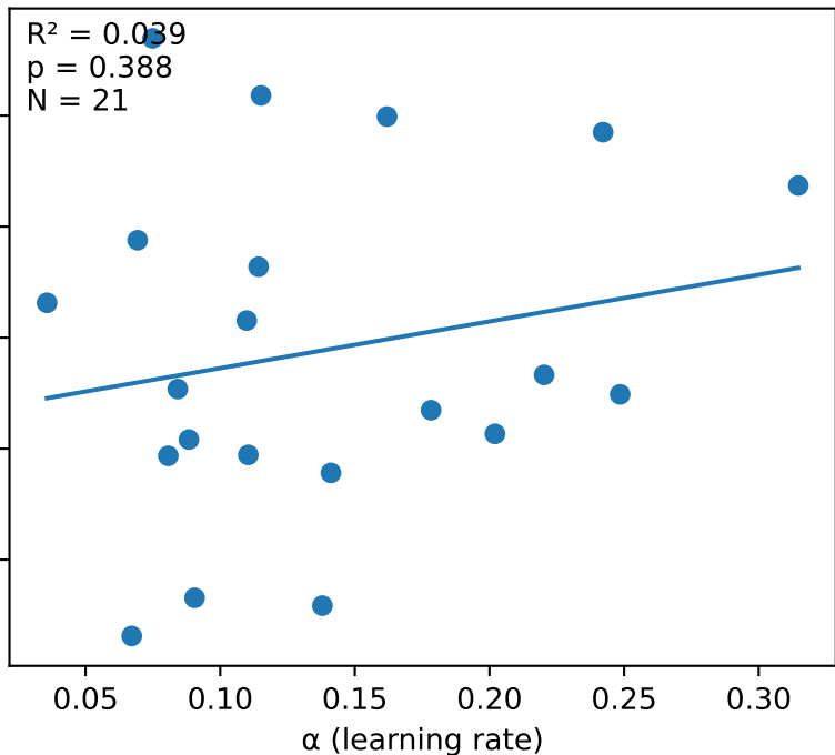
v_z_AttentionW:C(OVcate)[high]
