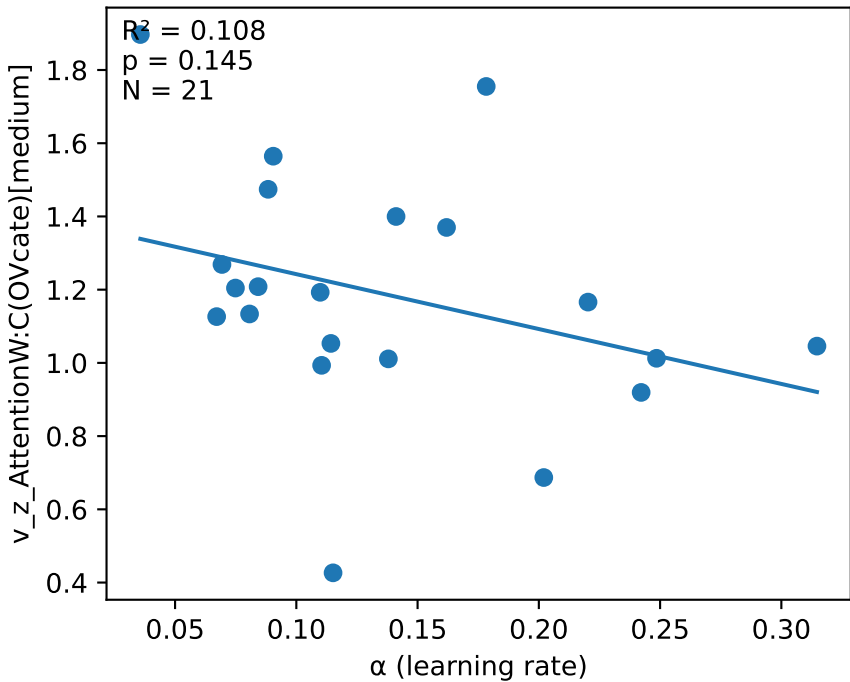
v_z_AttentionW:C(OVcate)[medium]
