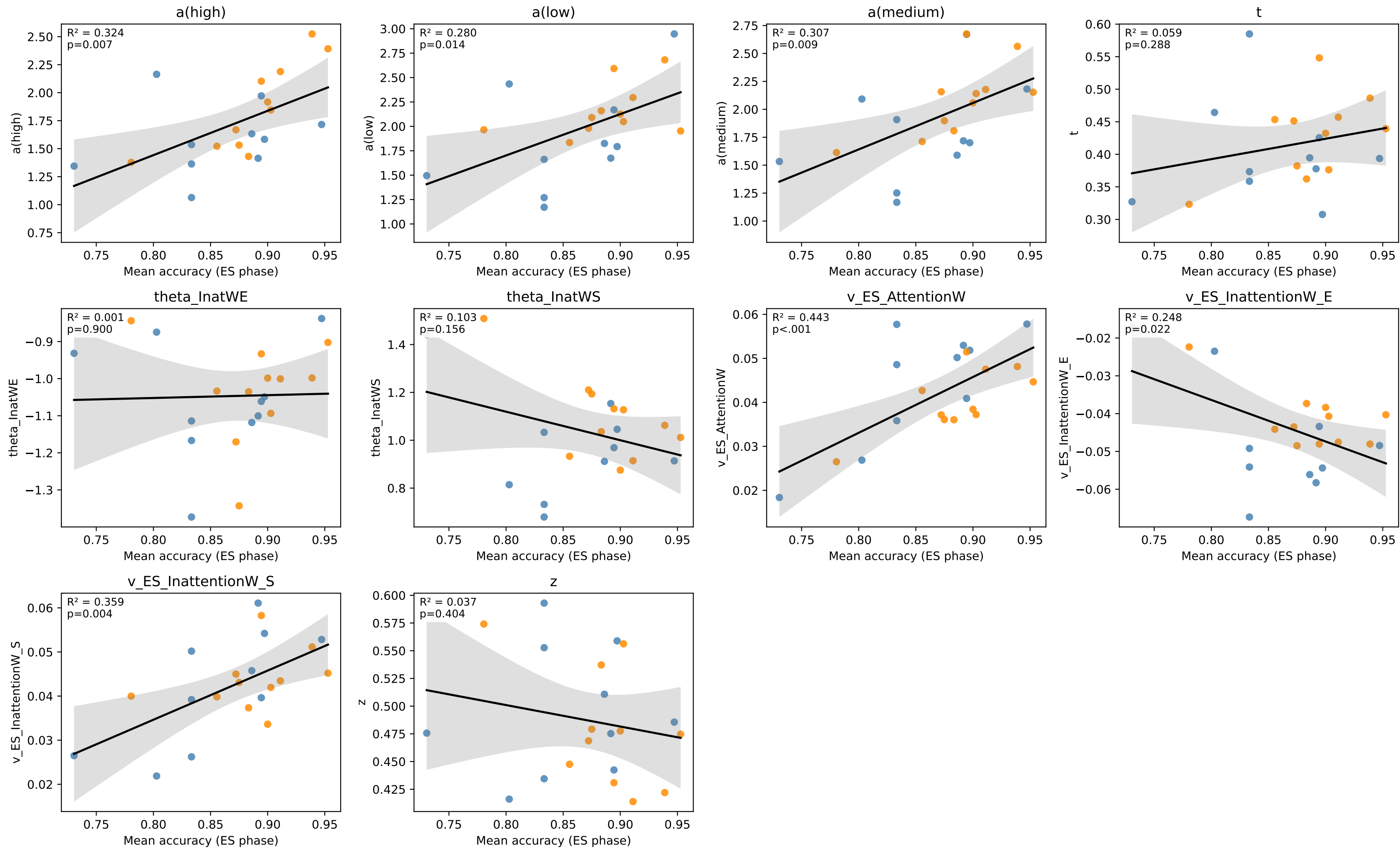
ES accuracy vs aDDM parameters (colored by LE \alpha median split)
