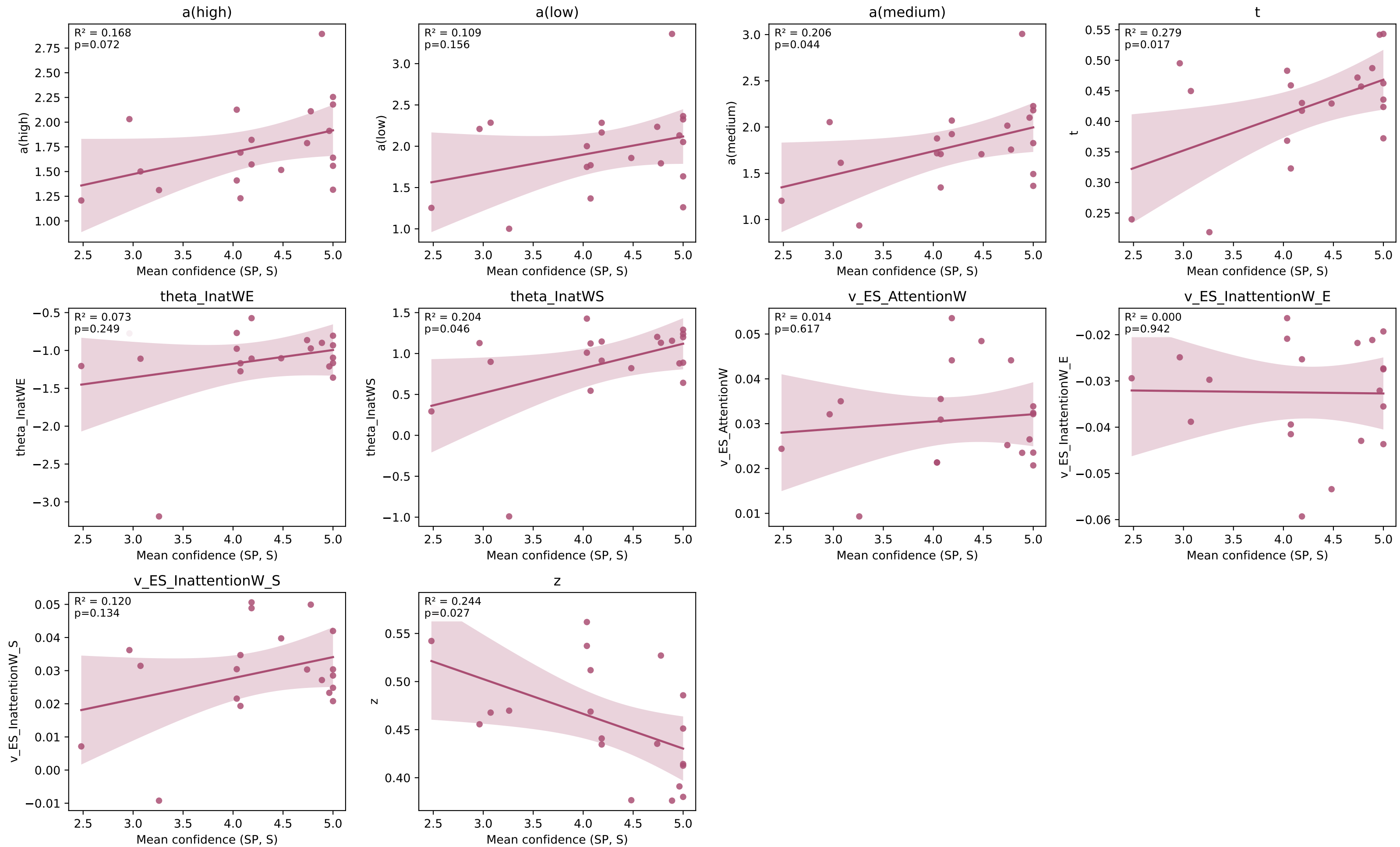
Correlations: SP confidence (S) vs aDDM parameters
