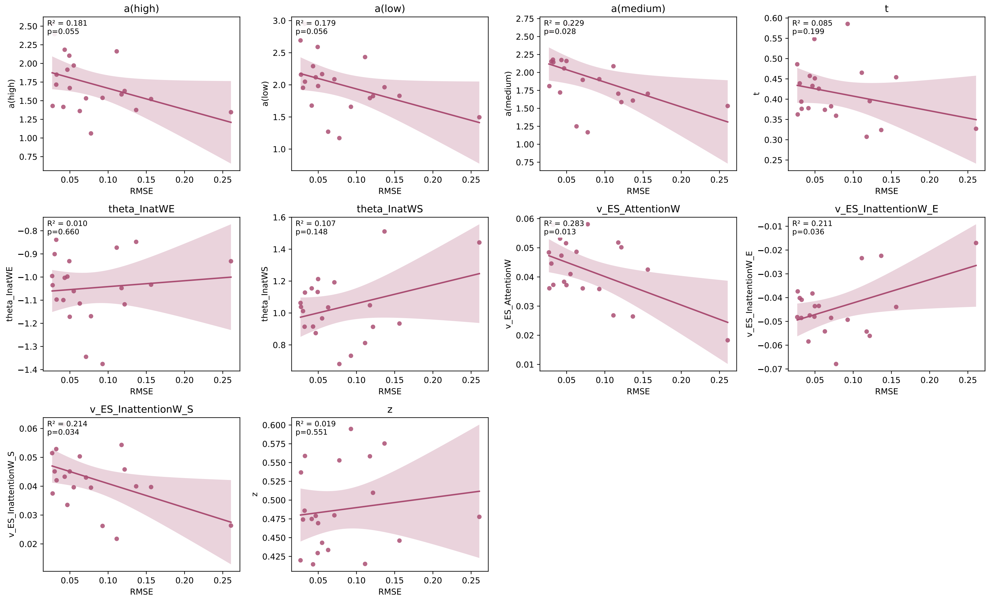
Correlations: SP RMSE (S) vs aDDM parameters
