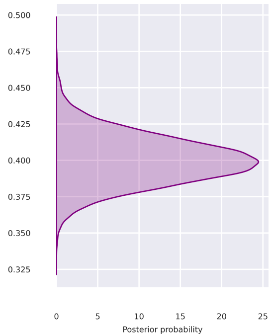
Non-dec. time p=0.000
