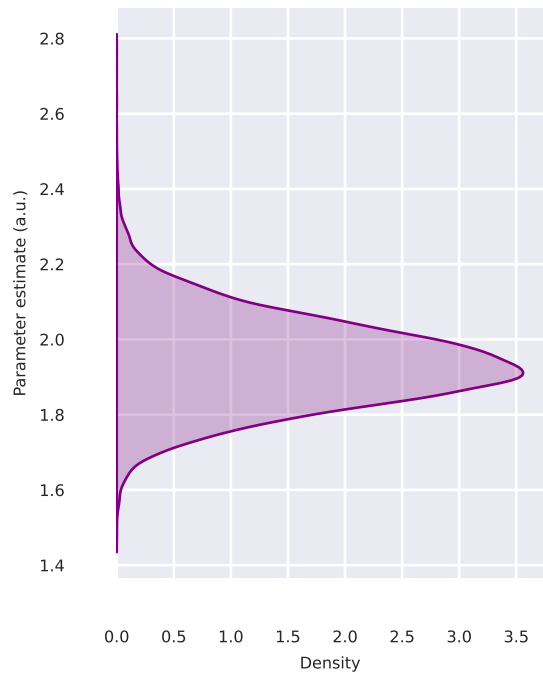
Boundary sep. p=0.000
