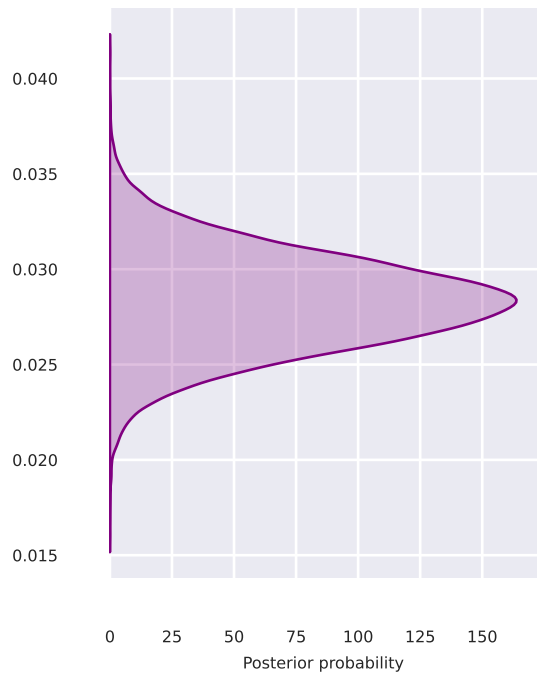
Drift InattentionW p=0.000
