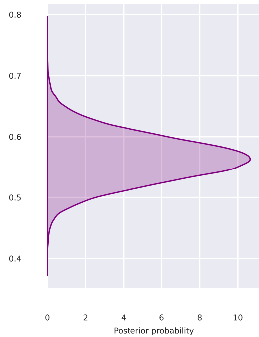
Intercept drift rate p=0.000
