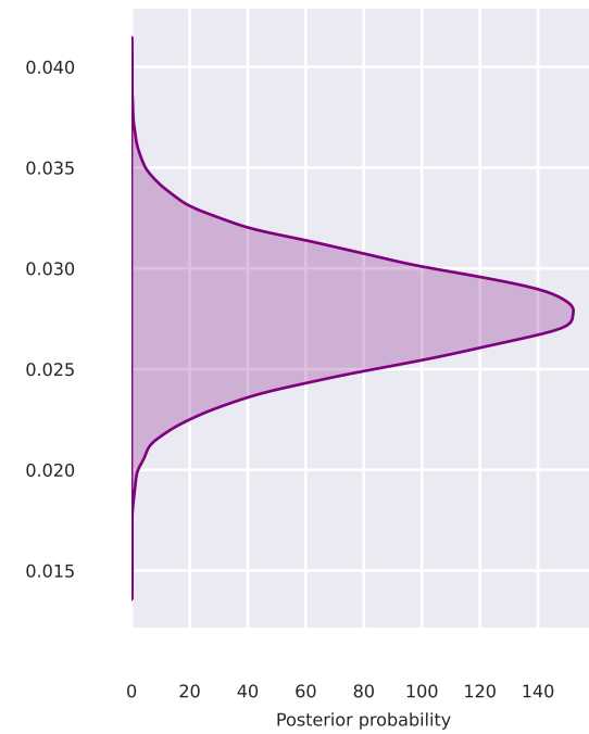
Drift AttentionW p=0.000
