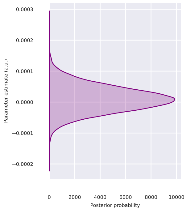
Drift gazeSE p=0.413
