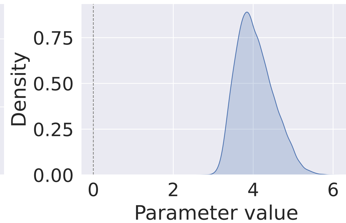
Boundary sep.
