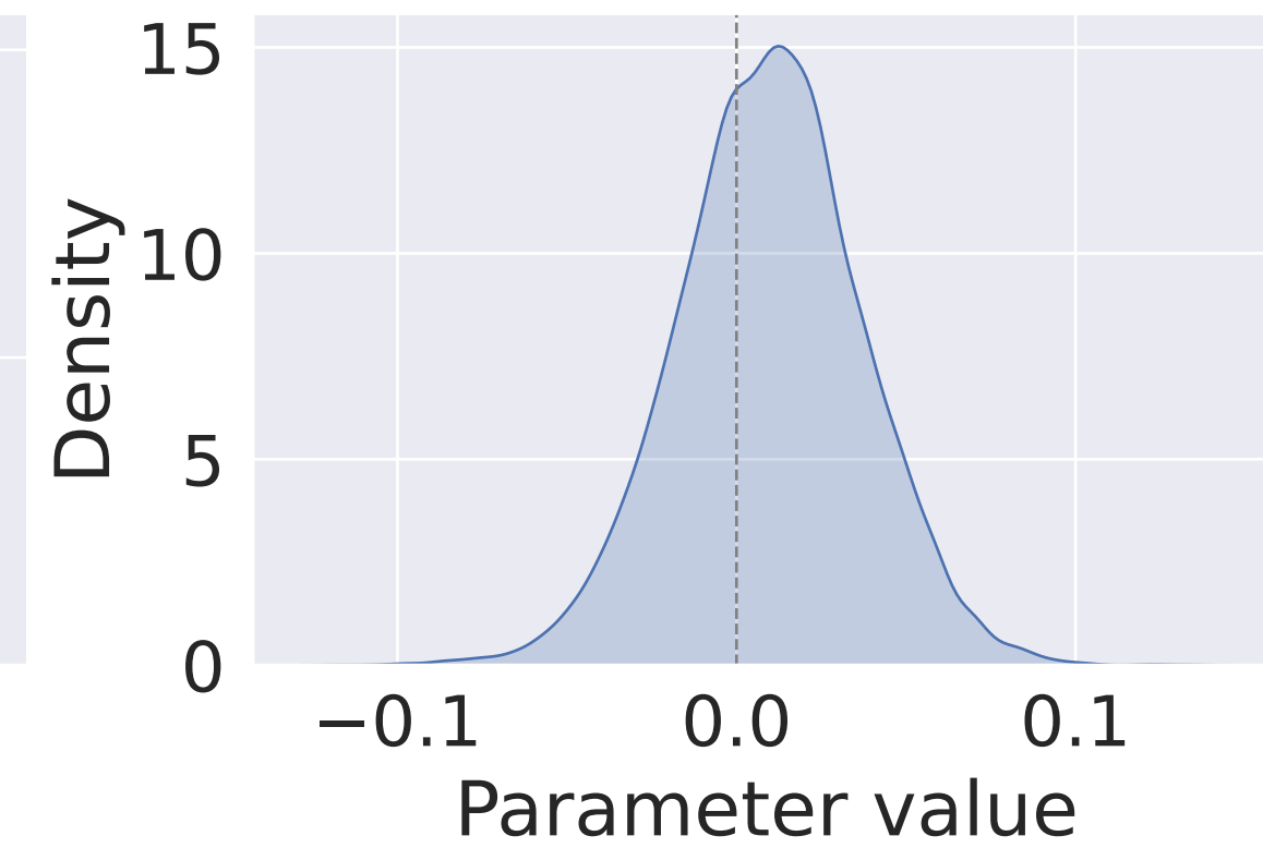
Drift sv_pain_para
