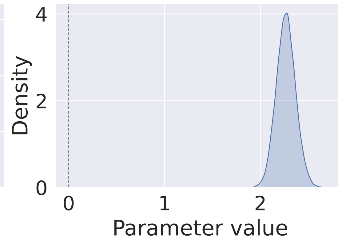
Drift Intercept
