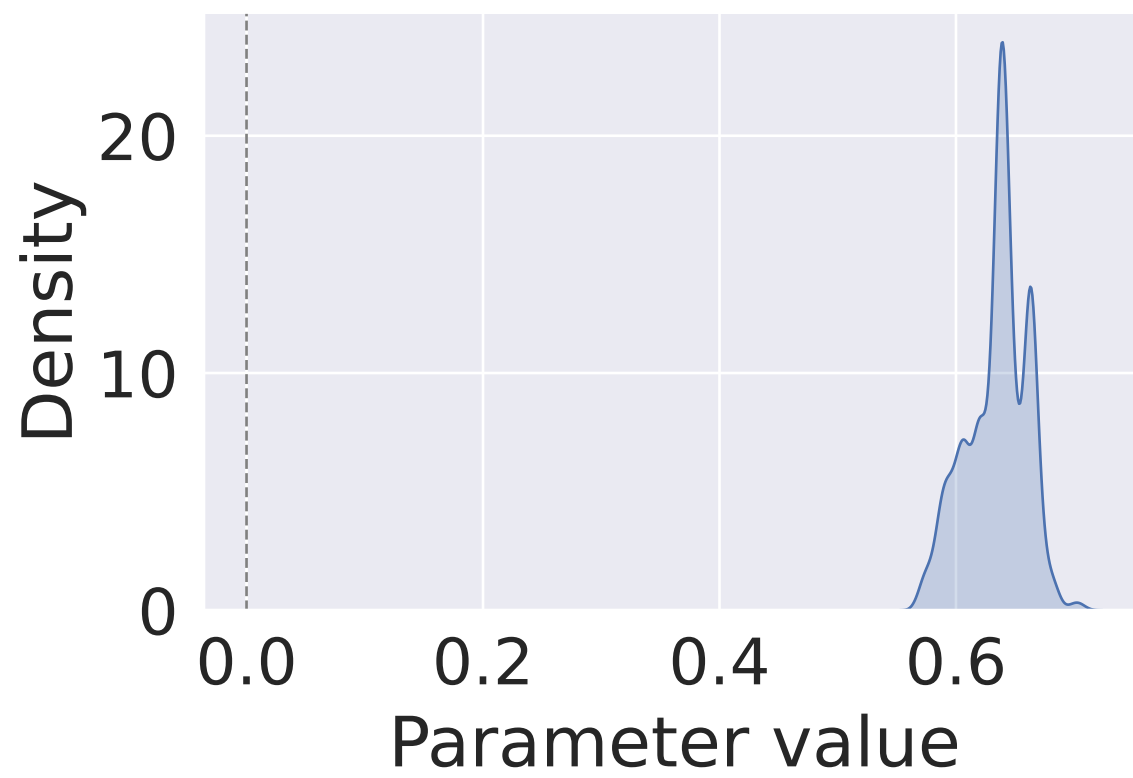
Starting point
