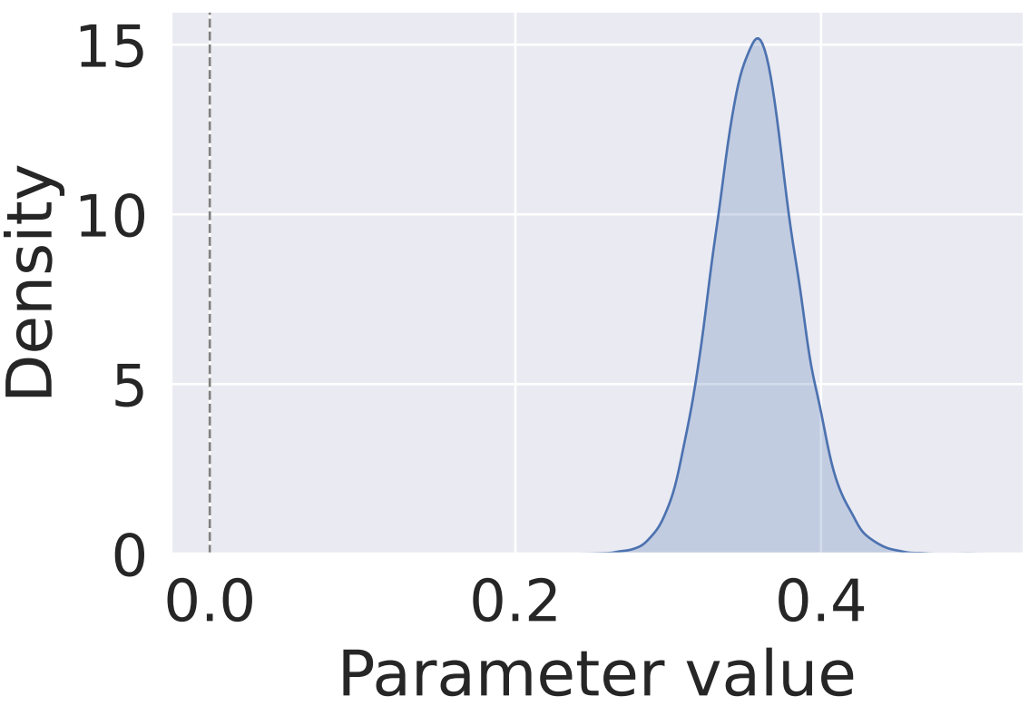
Non-dec. time
