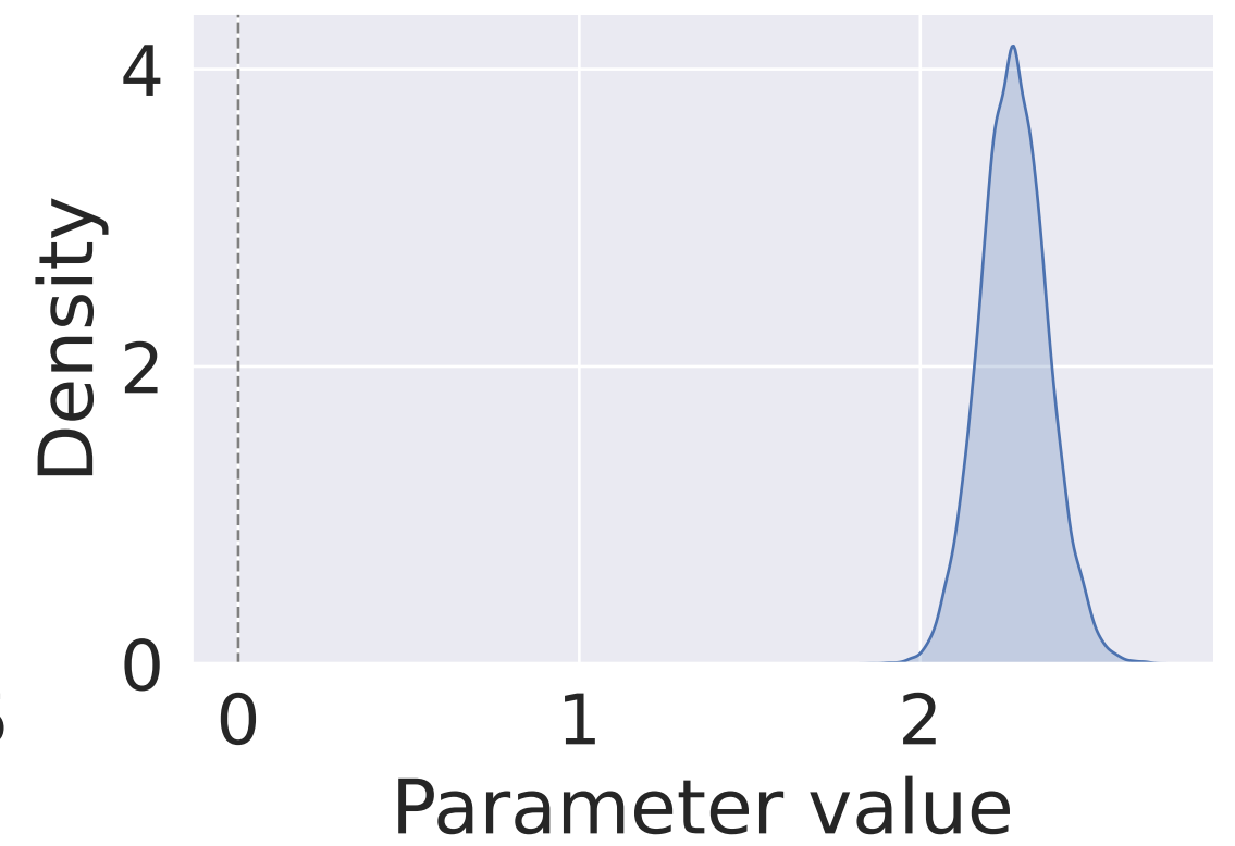
Drift Rate
