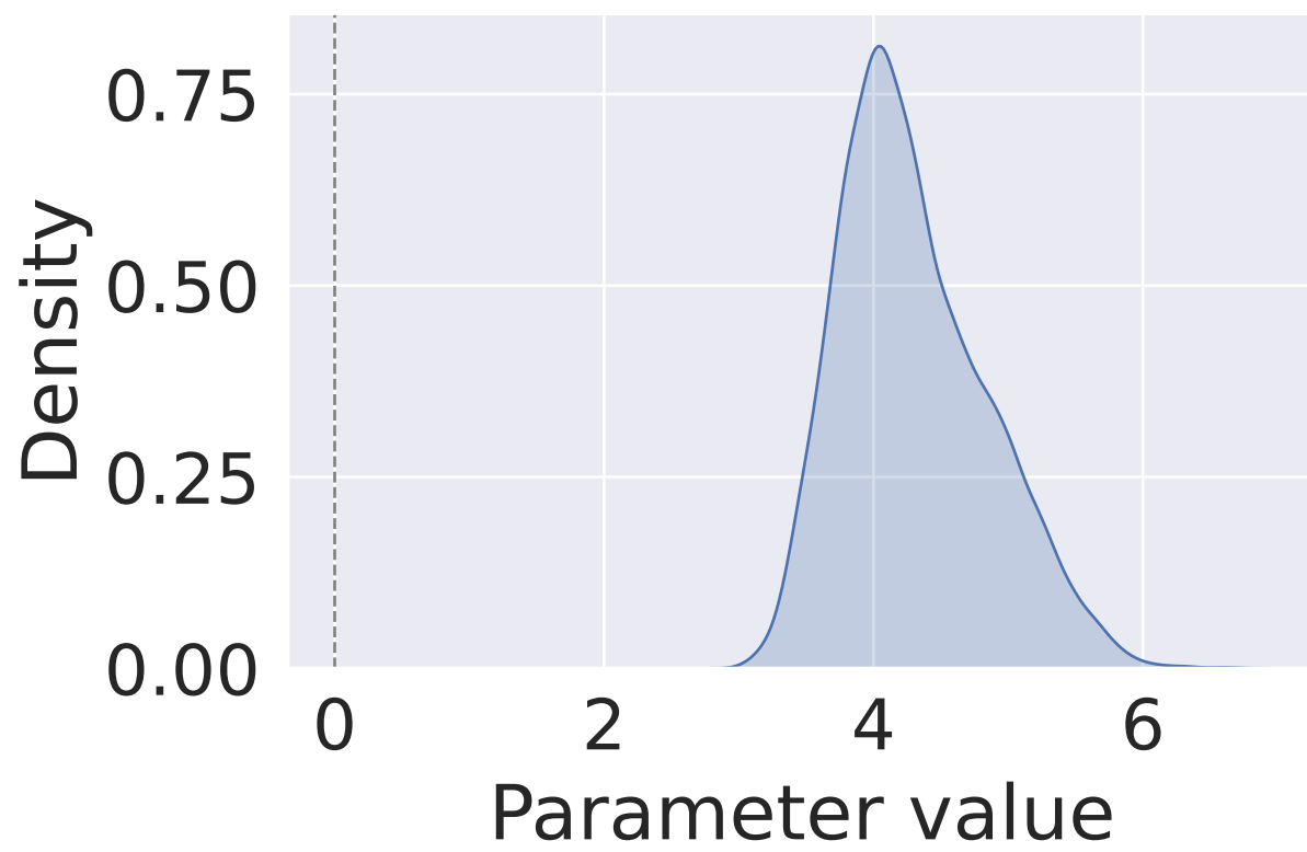
Threshold Intercept
