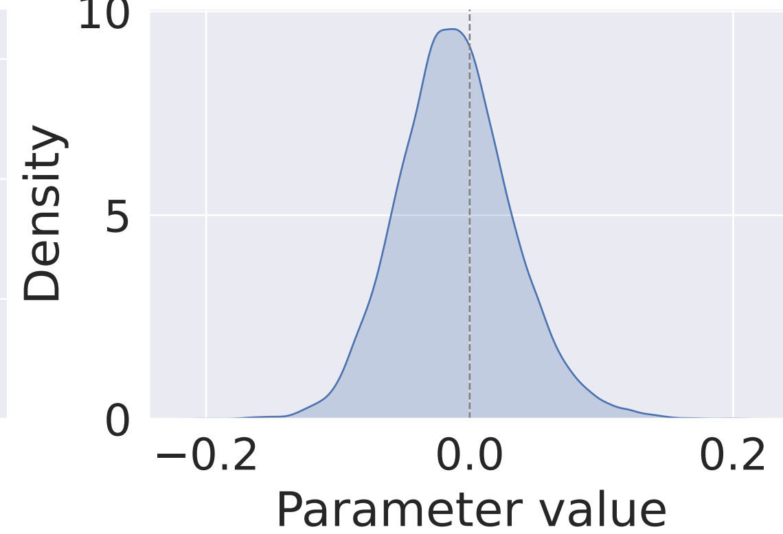
Threshold sv_pain_para
