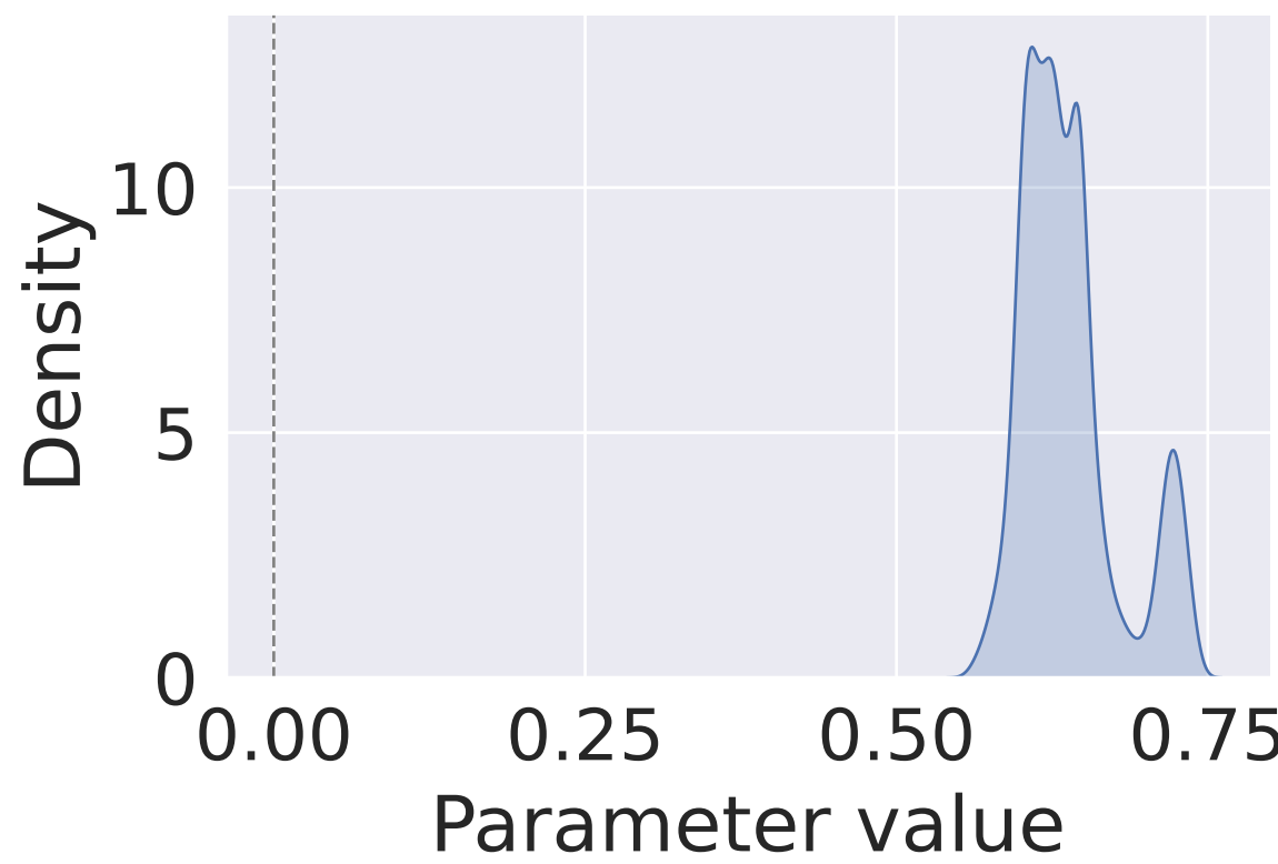
Starting point
