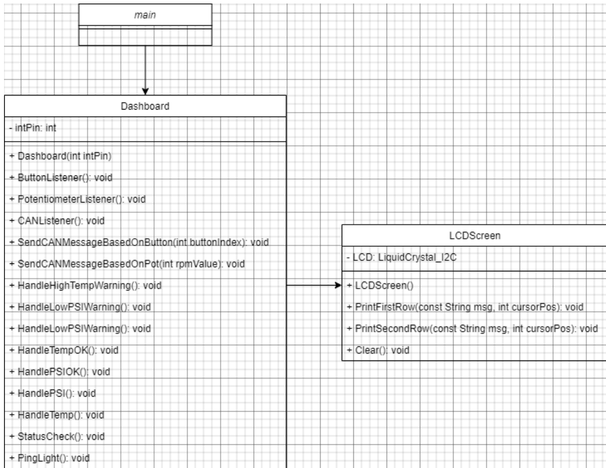
Figure 5: Dashboard ECU class diagram.
