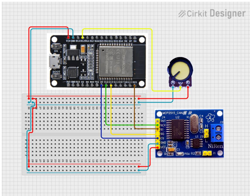
Figure 13: Wiring diagram of the Tires Node.
