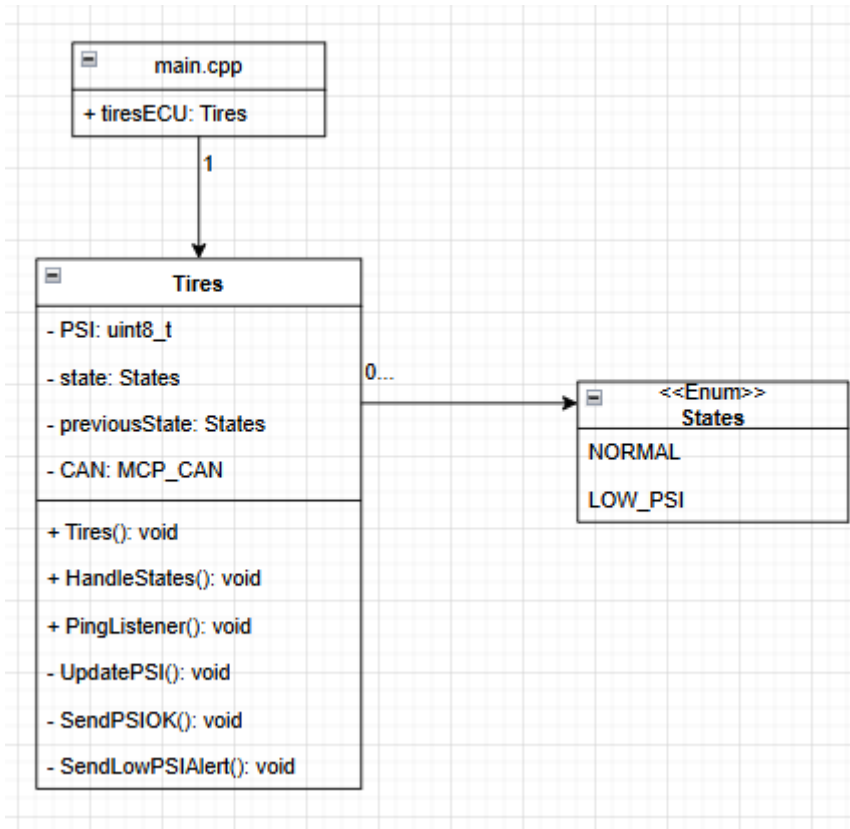
Figure 3: Tires ECU class diagram.
