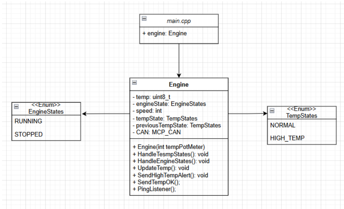
Figure 4: Engine ECU class diagram.
