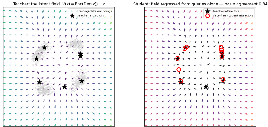
Figure 1: The object and the claim. Left: a teacher autoencoder’s latent field V(z) = E(D(z)) - z and the attractors training carved into it. Right: a data-free student’s field, regressed from field queries alone—no inputs, weights, or training data—with both attractor sets overlaid; basin agreement 0.84 this seed (Table 1).
