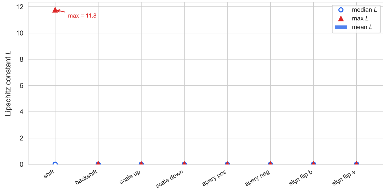
Fig. 4 — Lipschitz Constants per Operator (mean, median, max)
