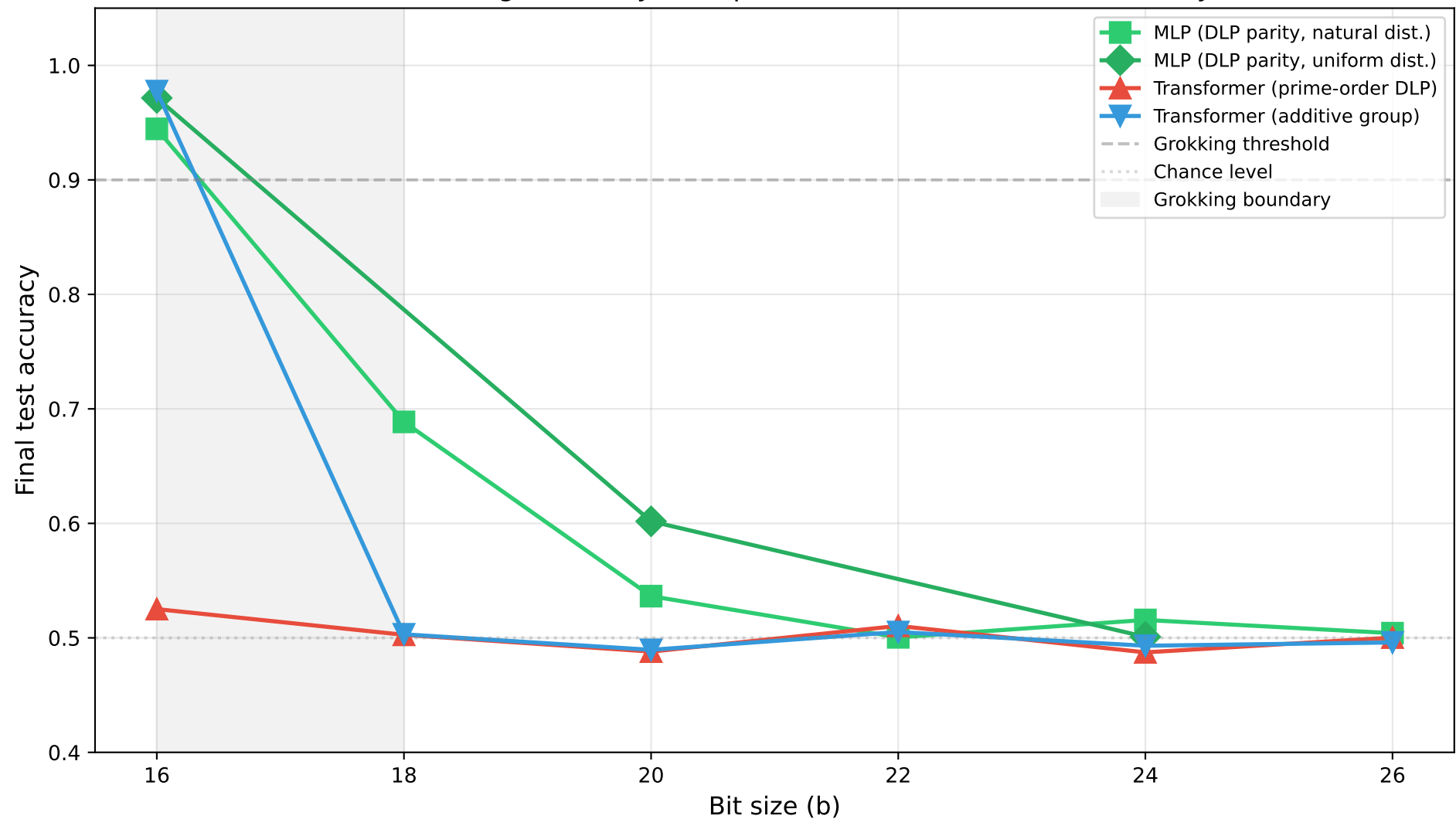
The Grokking Boundary: Group Structure Determines Learnability
