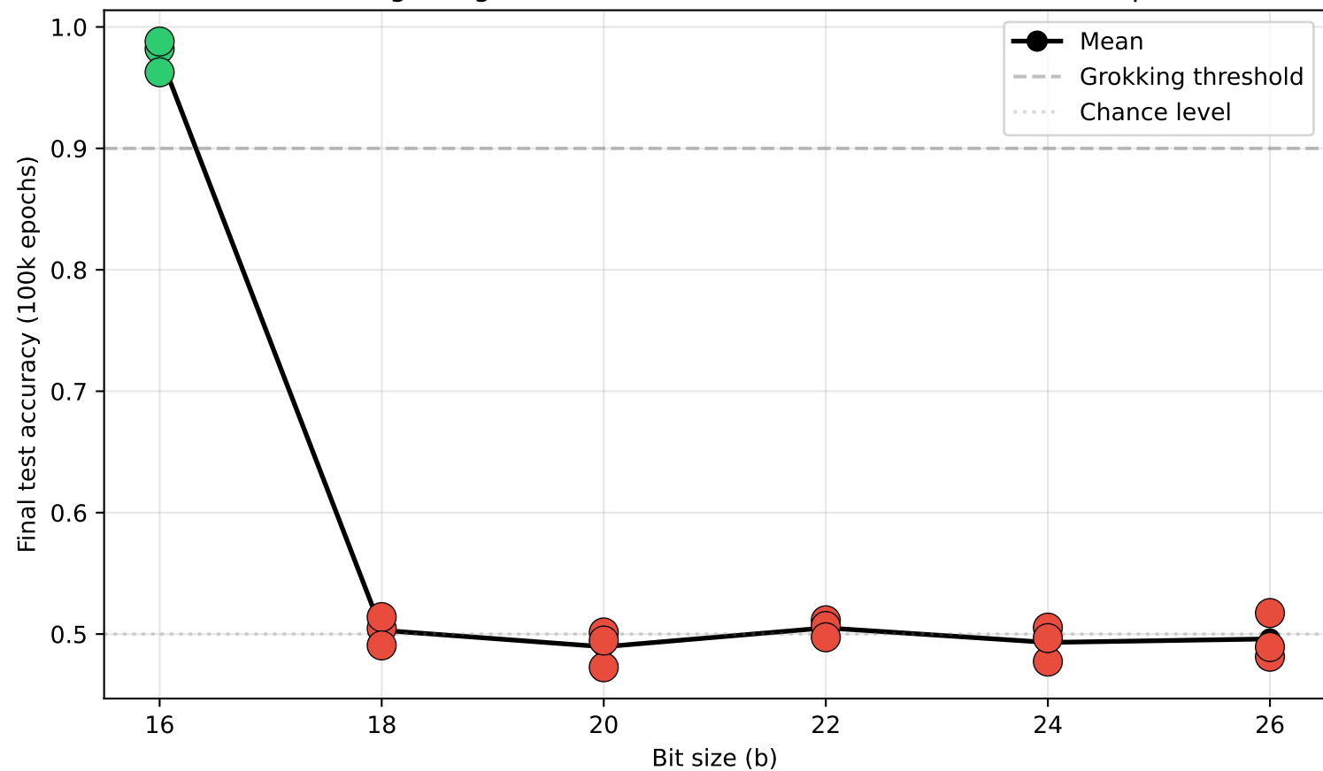
Grokking Bridge: Bit-Tokenizer Transformer on Additive Group
