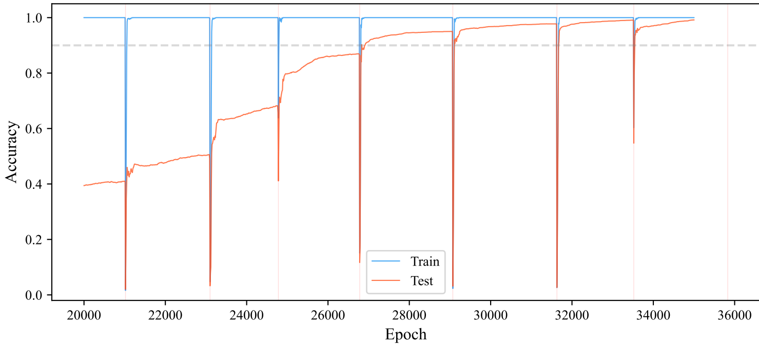
Slingshot Events During Grokking Transition (M04)
