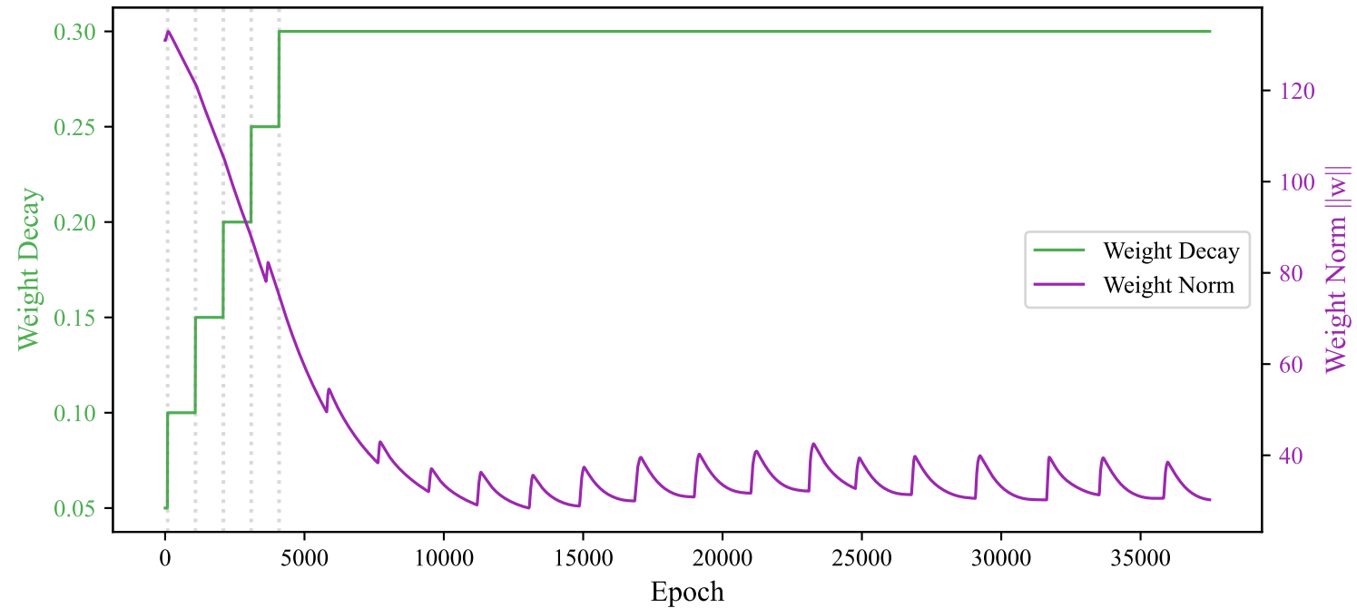
Progressive WD Schedule and Weight Norm Trajectory (M04)
