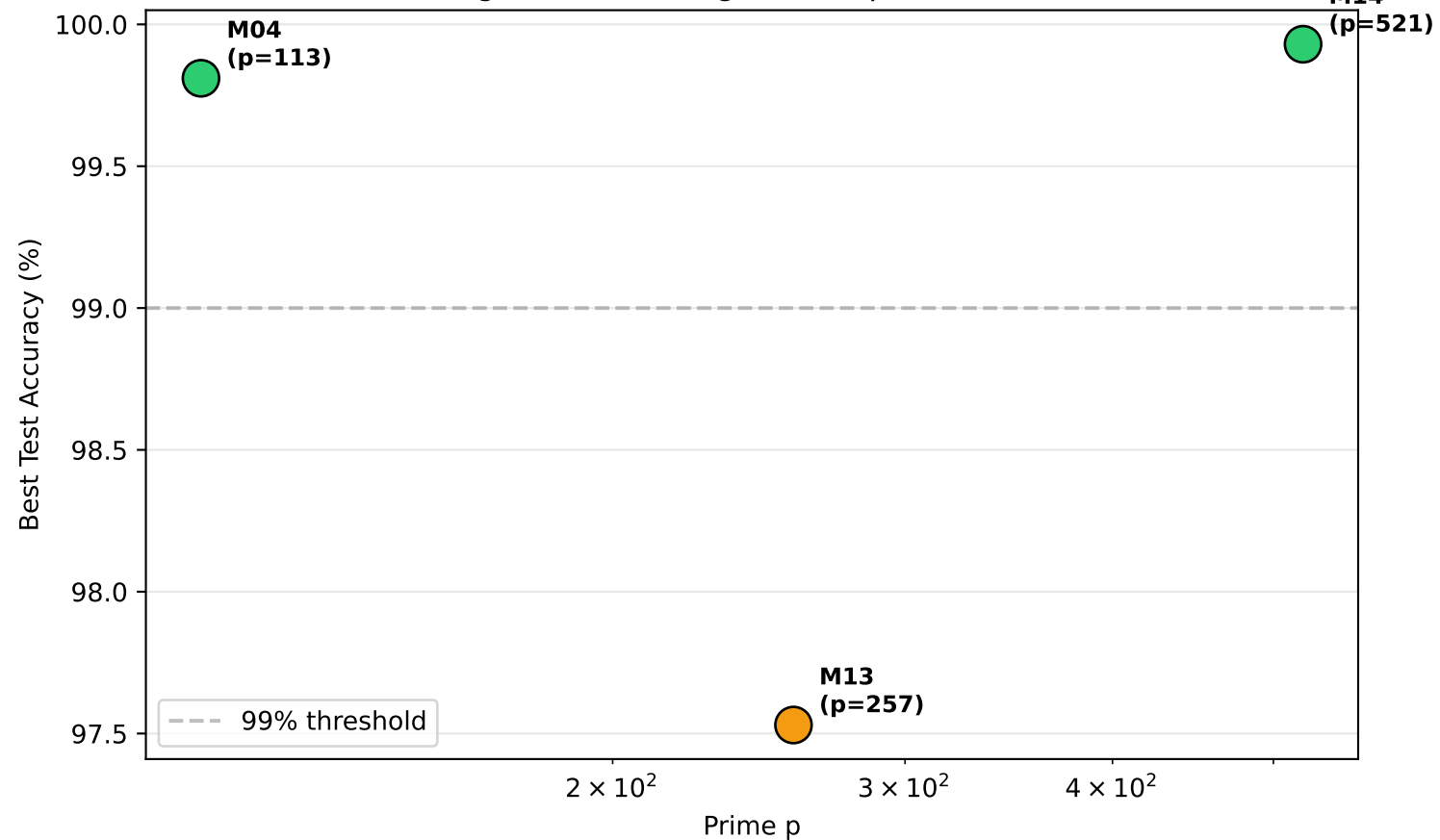
Large-Prime Scaling (RAW representation)
