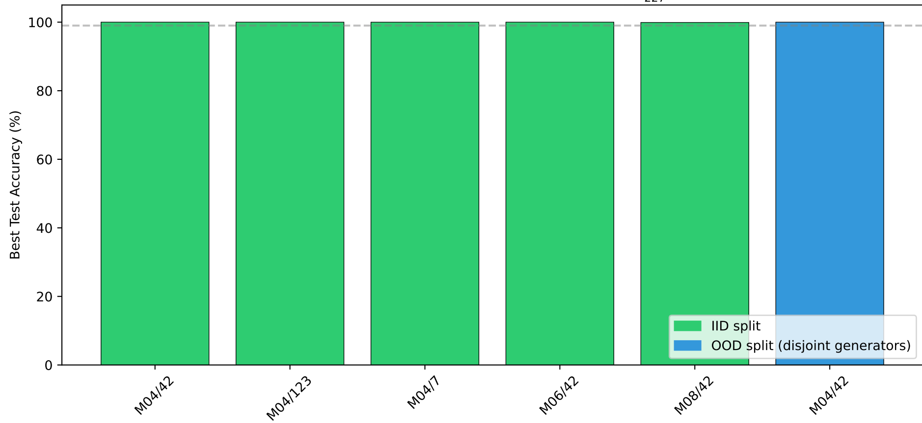
Prime-Order DLP (order-113 subgroup of \mathbb{F}_{227}^* )
