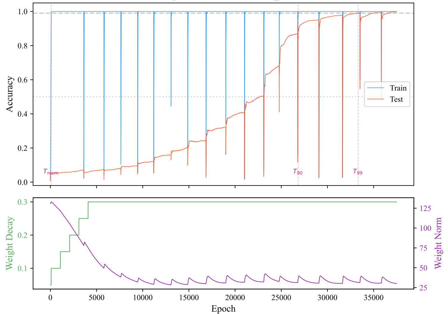
M04 (427k params, p = 113 , train\_frac=0.30)
